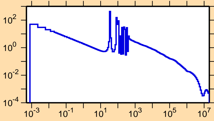
\sigma vs. E for ^{113}\text{Rh}(n,\gamma)
