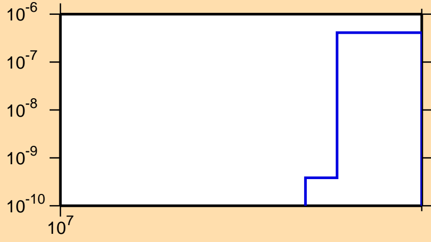
\sigma vs. E for ^{113}\text{Rh}(n,nt)
