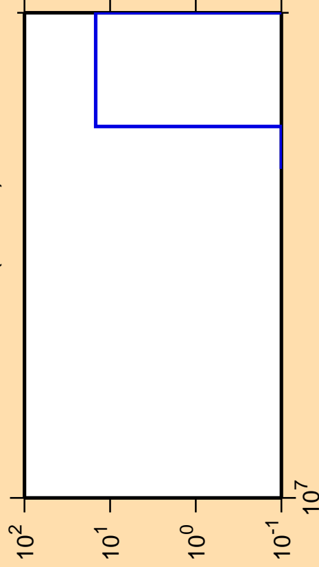
\Delta\sigma/\sigma vs. E for ^{113}\text{Rh}(n,2n\alpha)
