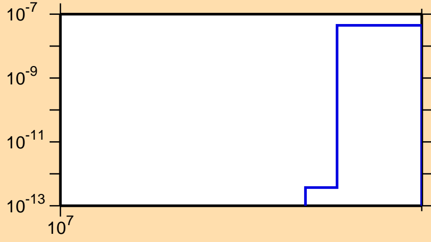
\sigma vs. E for ^{113}\text{Rh}(n,\text{nd})
