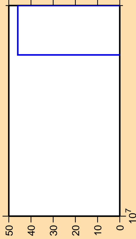
\Delta\sigma/\sigma vs. E for ^{113}\text{Rh}(n,2np)
