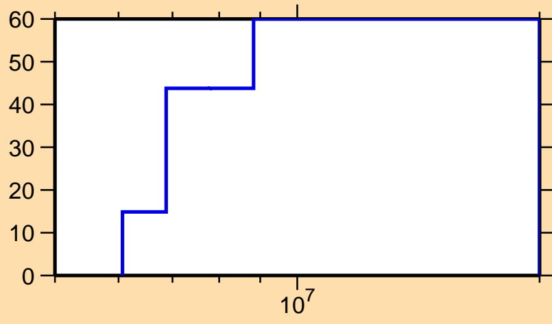
\Delta\sigma/\sigma vs. E for ^{113}\text{Rh}(n,n\text{cont.})
