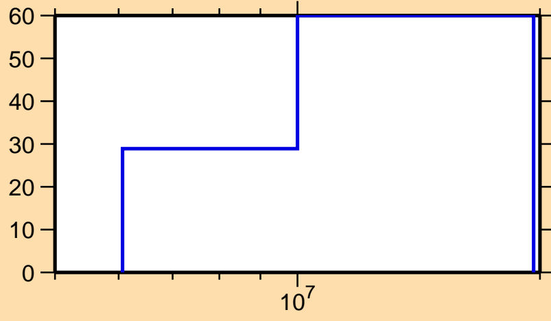
\Delta\sigma/\sigma vs. E for ^{113}\text{Rh}(n,ncont.)
