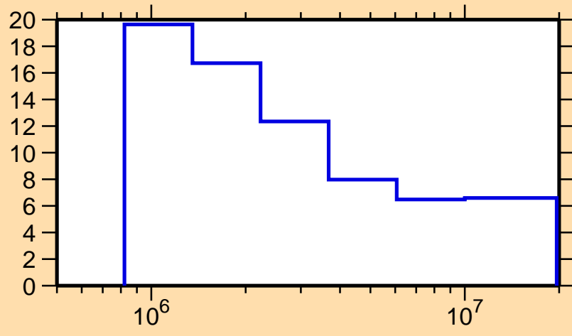
\Delta\sigma/\sigma vs. E for ^{114}\text{Rh}(n,n\text{nonel.})
