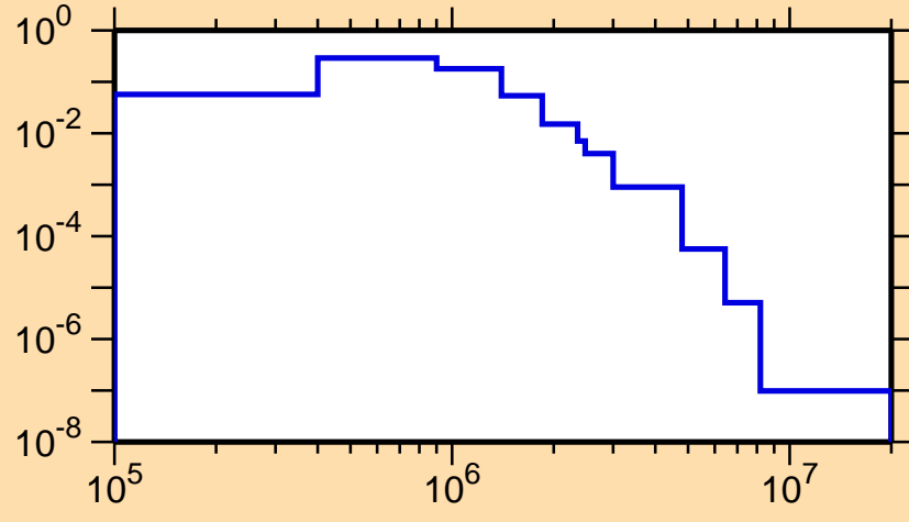
\sigma vs. E for ^{114}\text{Rh}(n,n_3)
