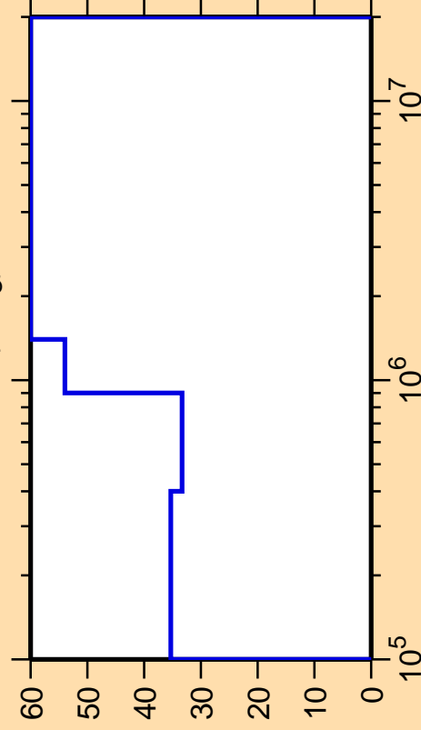
\Delta\sigma/\sigma vs. E for ^{114}\text{Rh}(n,n_3)
