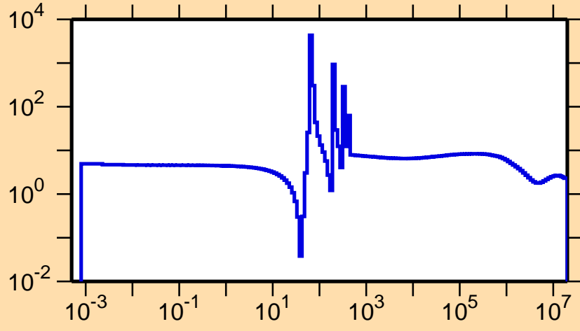
\sigma vs. E for ^{114}\text{Rh}(n,\text{el.})
