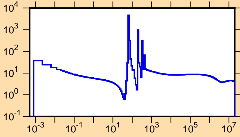
\sigma vs. E for ^{114}\text{Rh}(n,\text{tot.})
