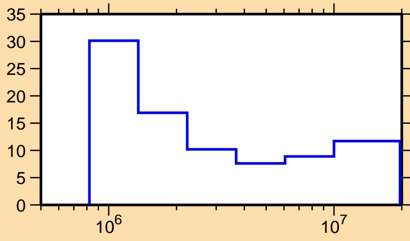
\Delta\sigma/\sigma vs. E for ^{114}\text{Rh}(n,n\text{onel.})
