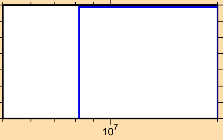
\sigma vs. E for ^{114}\text{Rh}(n,np)
