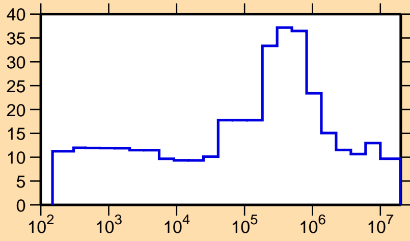
\Delta\sigma/\sigma vs. E for ^{200}\text{Rn}(n,el.)
