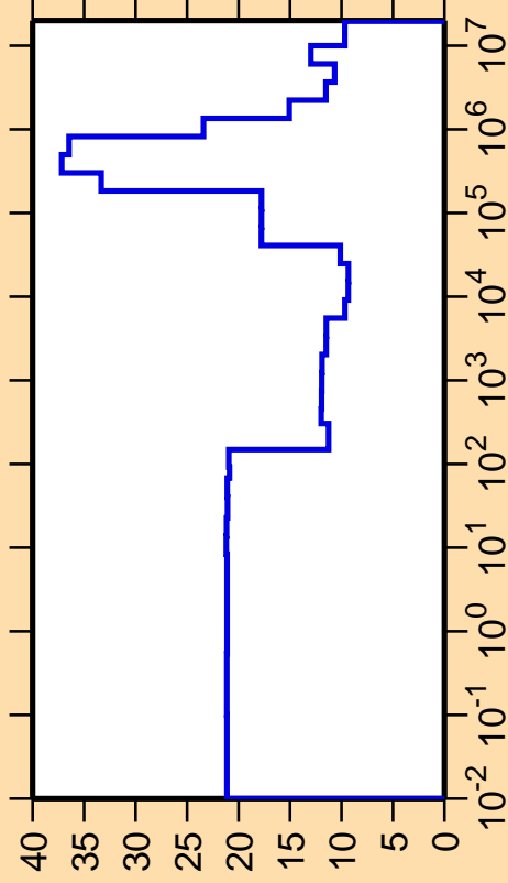
\Delta\sigma/\sigma vs. E for ^{200}\text{Rn}(n,\text{el.})
