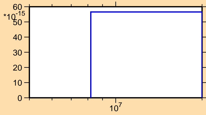
\sigma vs. E for ^{200}\text{Rn}(\text{mt } 34)
