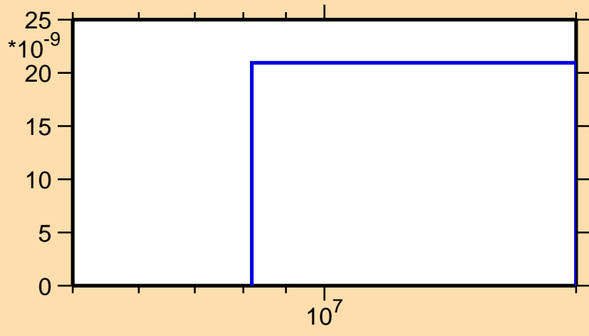
\sigma vs. E for ^{200}\text{Rn}(n,\text{pd})
