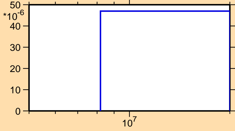
\sigma vs. E for ^{200}\text{Rn}(n,t)
