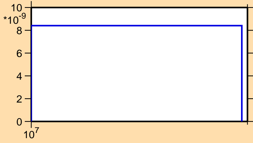
\sigma vs. E for ^{201}\text{Rn}(n,\text{nd})
