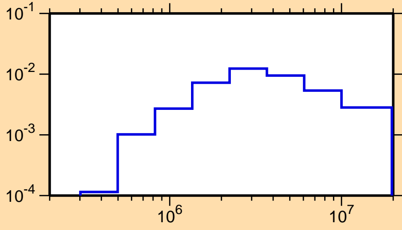
\sigma vs. E for ^{201}\text{Rn}(n,n_4)
