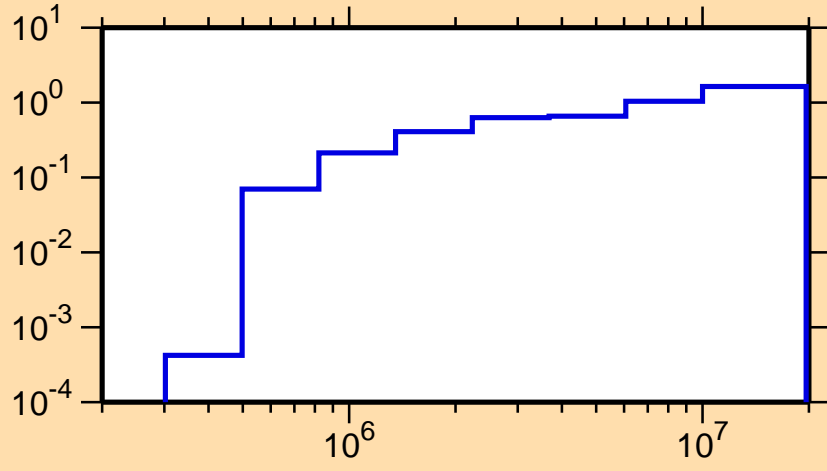
\sigma vs. E for ^{201}\text{Rn}(n,\text{inel.})
