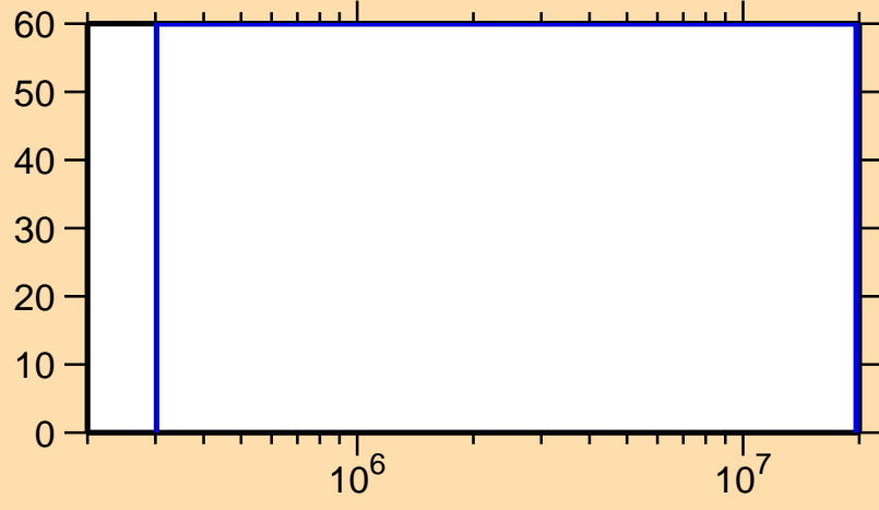
\Delta\sigma/\sigma vs. E for ^{201}\text{Rn}(n,n_1)
