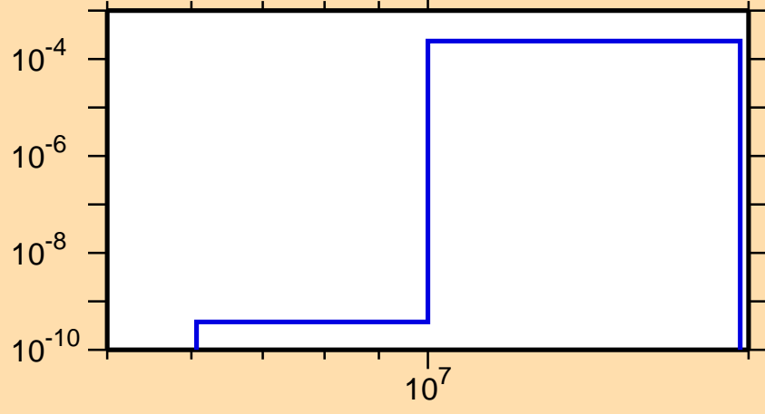
\sigma vs. E for ^{201}\text{Rn}(n,t)
