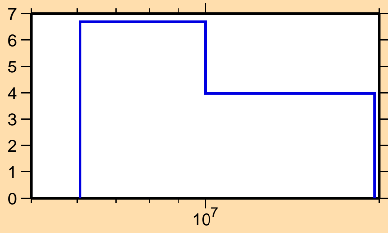
\Delta\sigma/\sigma vs. E for ^{201}\text{Rn}(n,\text{nonel.})
