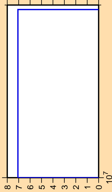
\Delta\sigma/\sigma vs. E for ^{201}\text{Rn}(n,3n\alpha)
