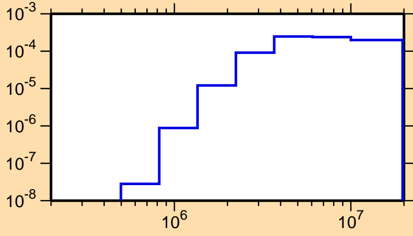
\sigma vs. E for ^{201}\text{Rn}(n,n_2)
