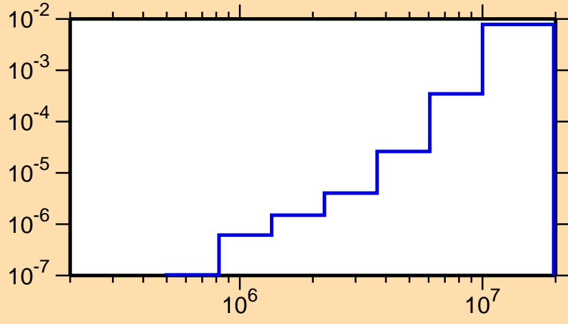
\sigma vs. E for ^{201}\text{Rn}(n,n\alpha)
