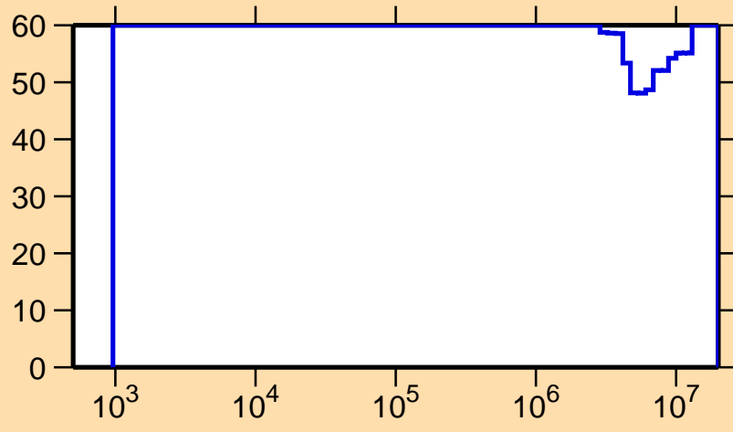
\Delta\sigma/\sigma vs. E for ^{201}\text{Rn}(n,ncont.)
