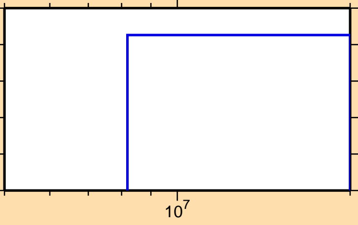
\sigma vs. E for ^{201}\text{Rn}(n,2n\alpha)
