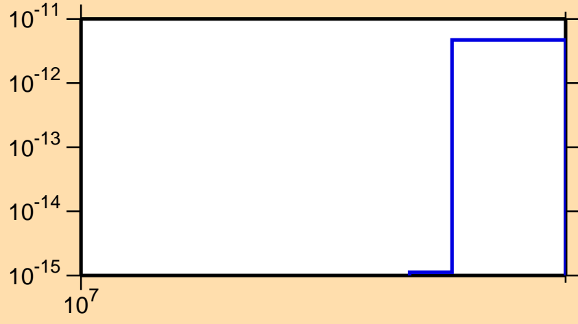
\sigma vs. E for ^{202}\text{Rn}(n,nt)
