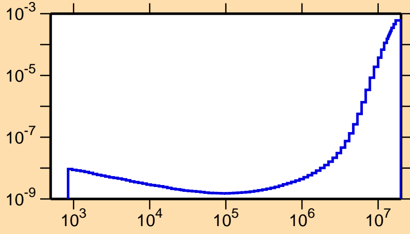
\sigma vs. E for ^{202}\text{Rn}(n,p\alpha)
