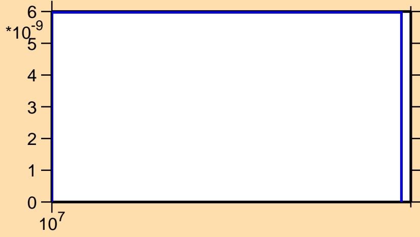
\sigma vs. E for ^{202}\text{Rn}(n,2np)
