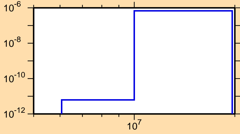
\sigma vs. E for ^{202}\text{Rn}(n,\text{He}3)
