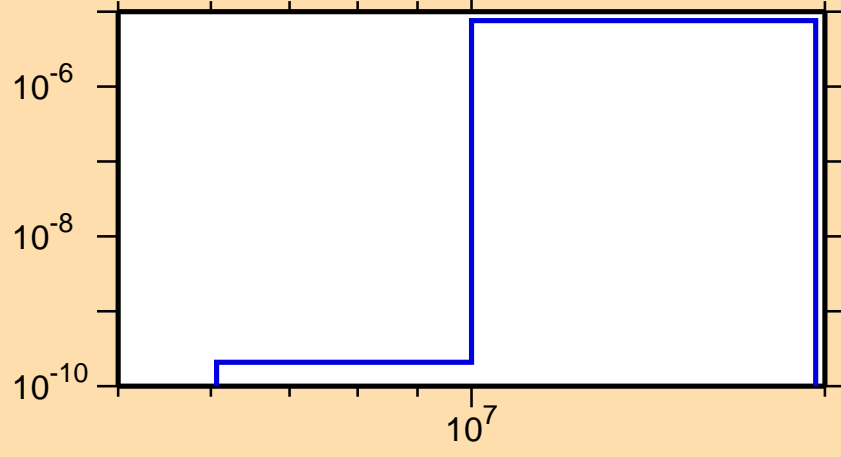
\sigma vs. E for ^{202}\text{Rn}(\text{mt117})
