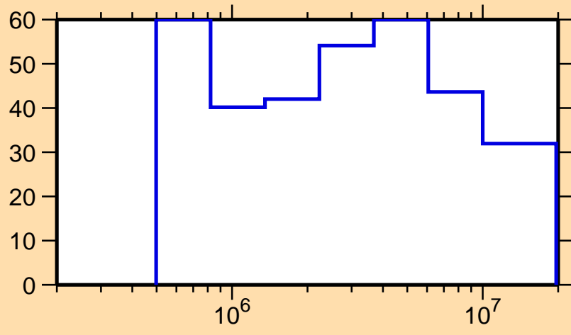
\Delta\sigma/\sigma vs. E for ^{202}\text{Rn}(n,\text{inel.})
