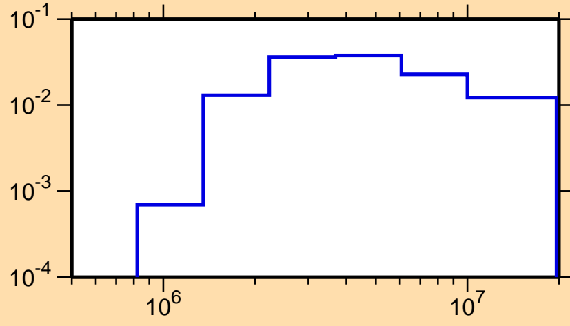
\sigma vs. E for ^{202}\text{Rn}(n,n_3)
