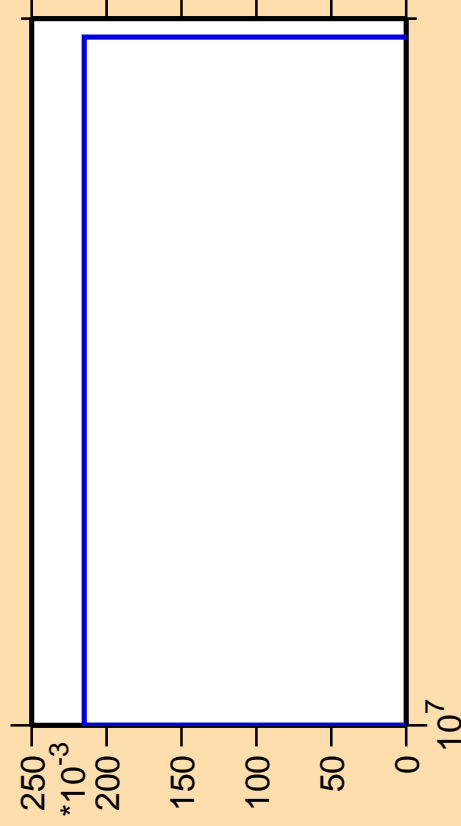
\Delta\sigma/\sigma vs. E for ^{202}\text{Rn} (mt 34)
