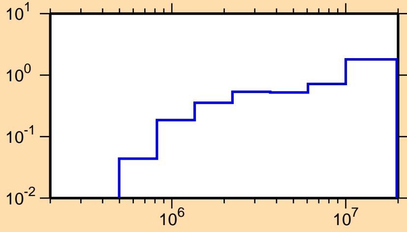
\sigma vs. E for ^{202}\text{Rn}(n,\text{inel.})
