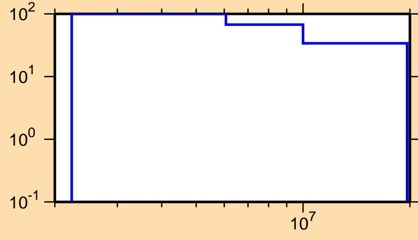
\Delta\sigma/\sigma vs. E for ^{202}\text{Rn}(n,n\text{cont.})
