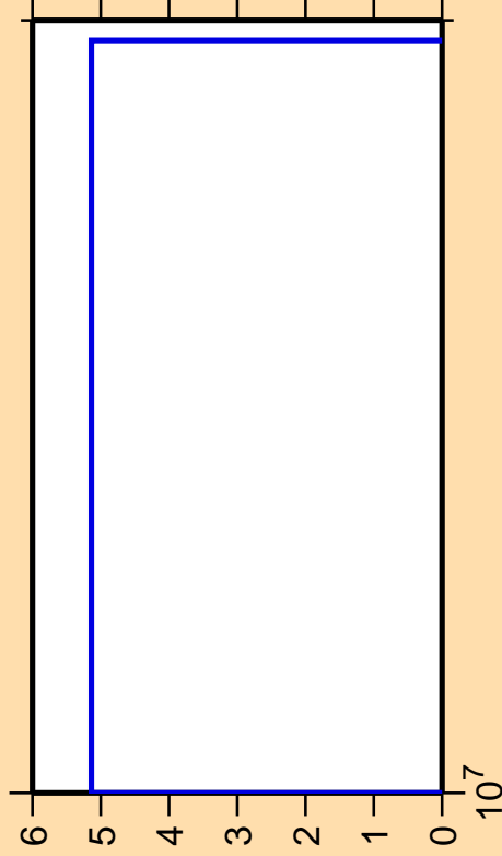
\Delta\sigma/\sigma vs. E for ^{202}\text{Rn}(n,pt)
