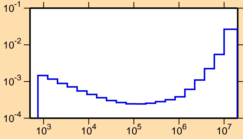
\sigma vs. E for ^{202}\text{Rn}(n,\alpha)
