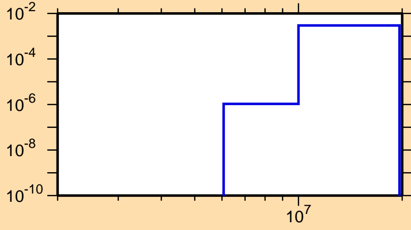
\sigma vs. E for ^{202}\text{Rn}(n,d)
