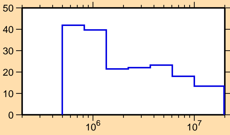
\Delta\sigma/\sigma vs. E for ^{202}\text{Rn}(n,\text{el.})
