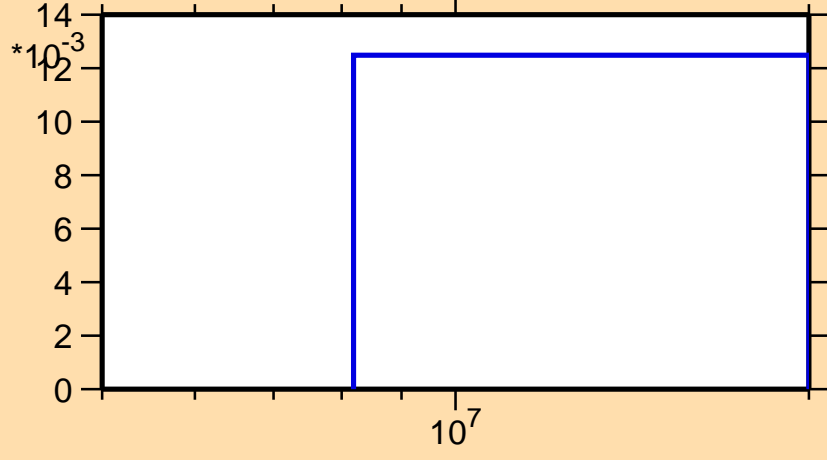
\sigma vs. E for ^{202}\text{Rn}(n,2n)
