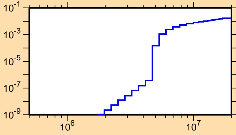
\sigma vs. E for ^{203}\text{Rn}(n,n\alpha)
