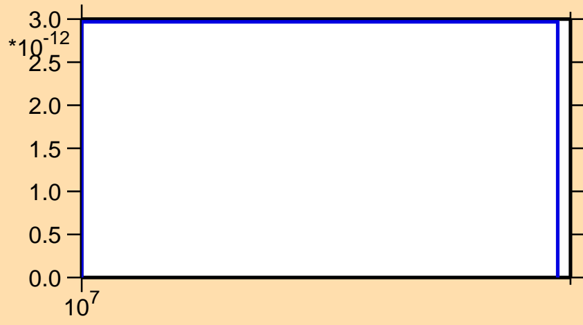
\sigma vs. E for ^{203}\text{Rn} (mt 34)
