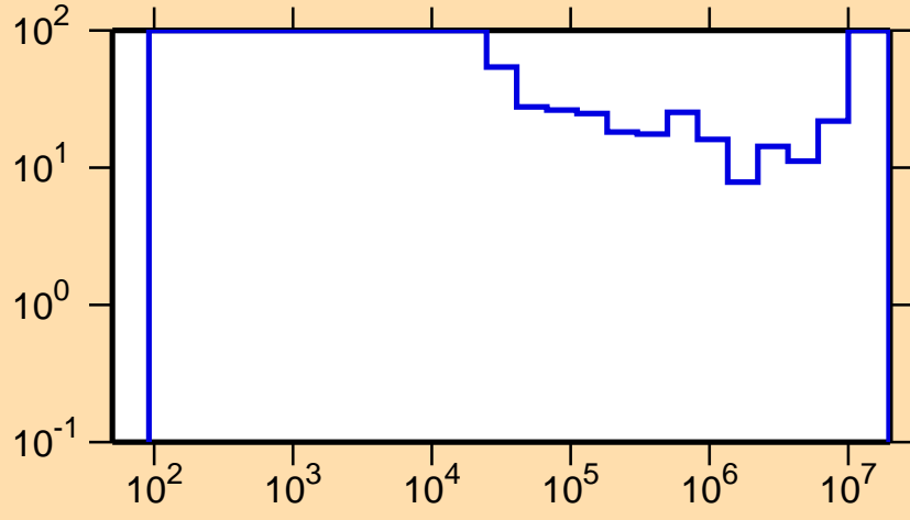
\Delta\sigma/\sigma vs. E for ^{203}\text{Rn}(n,\gamma)
