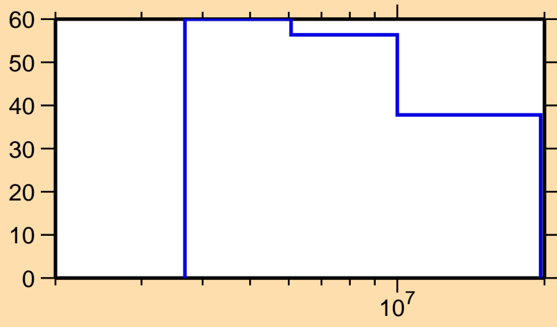
\Delta\sigma/\sigma vs. E for ^{203}\text{Rn}(n,n\text{cont.})
