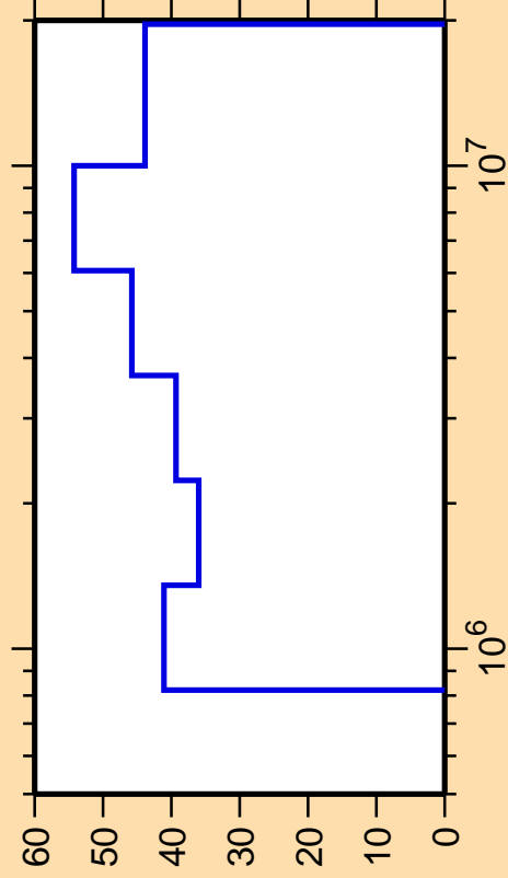
\Delta\sigma/\sigma vs. E for ^{203}\text{Rn}(n,\text{inel.})
