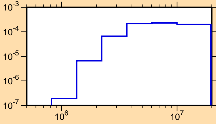
\sigma vs. E for ^{203}\text{Rn}(n,n_2)
