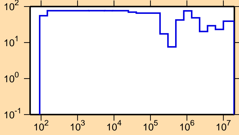
\Delta\sigma/\sigma vs. E for ^{203}\text{Rn}(n,\text{el.})
