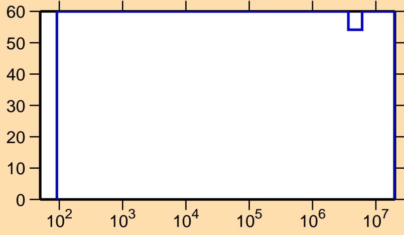
\Delta\sigma/\sigma vs. E for ^{203}\text{Rn}(n,p)
