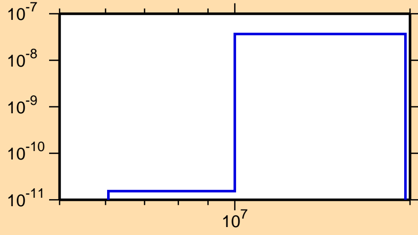
\sigma vs. E for ^{203}\text{Rn}(\text{mt117})
