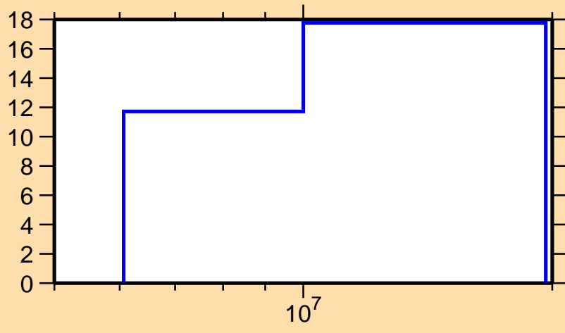
\Delta\sigma/\sigma vs. E for ^{203}\text{Rn}(n,\text{tot.})
