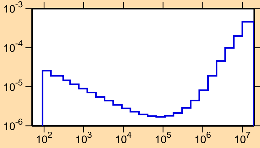
\sigma vs. E for ^{203}\text{Rn}(n,p\alpha)
