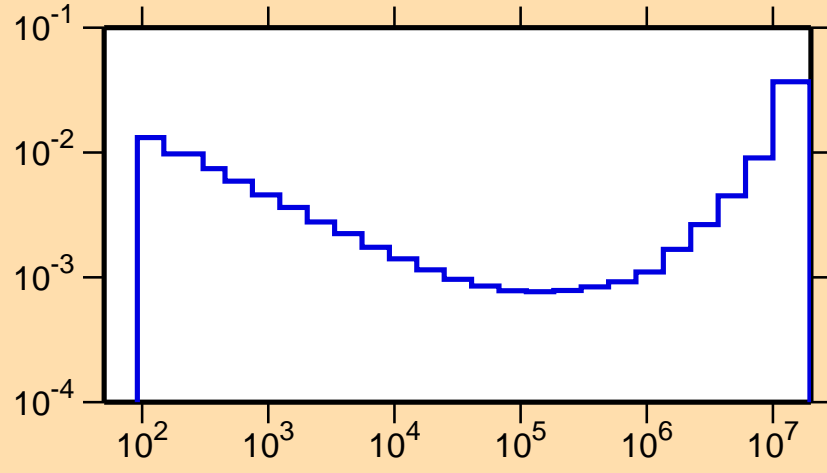
\sigma vs. E for ^{203}\text{Rn}(n,\alpha)
