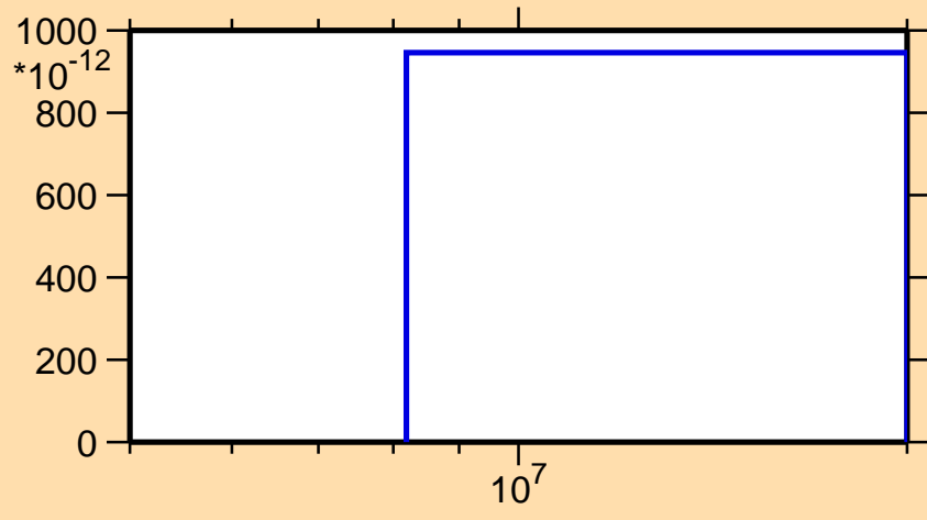
\sigma vs. E for ^{203}\text{Rn}(n,\text{pd})
