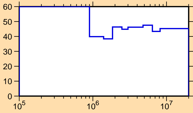
\Delta\sigma/\sigma vs. E for ^{203}\text{Rn}(n,n_1)
