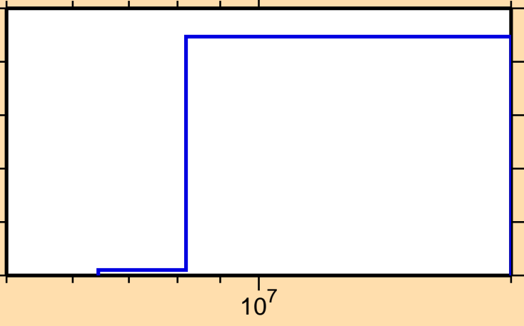
\sigma vs. E for ^{203}\text{Rn}(\text{mt117})
