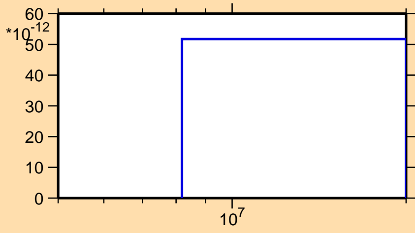
\sigma vs. E for ^{203}\text{Rn}(n,3n\alpha)
