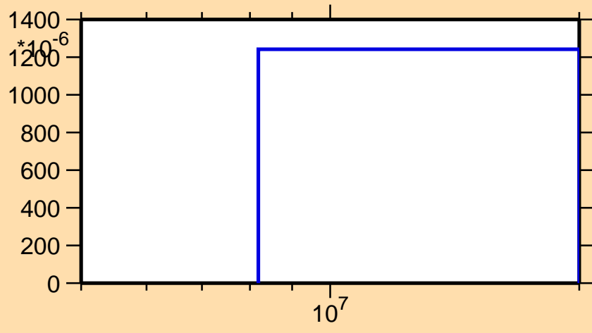
\sigma vs. E for ^{203}\text{Rn}(n,2n\alpha)
