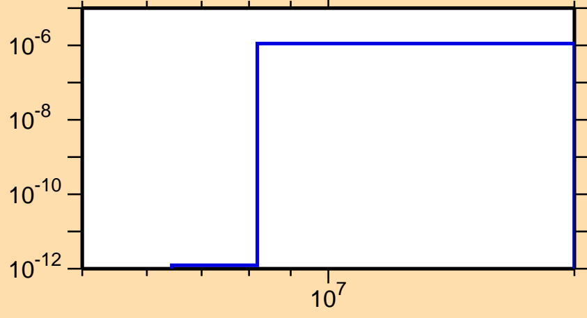
\sigma vs. E for ^{203}\text{Rn}(n,\text{He}3)
