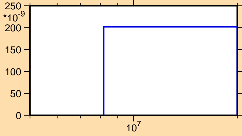
\sigma vs. E for ^{203}\text{Rn}(n,2np)
