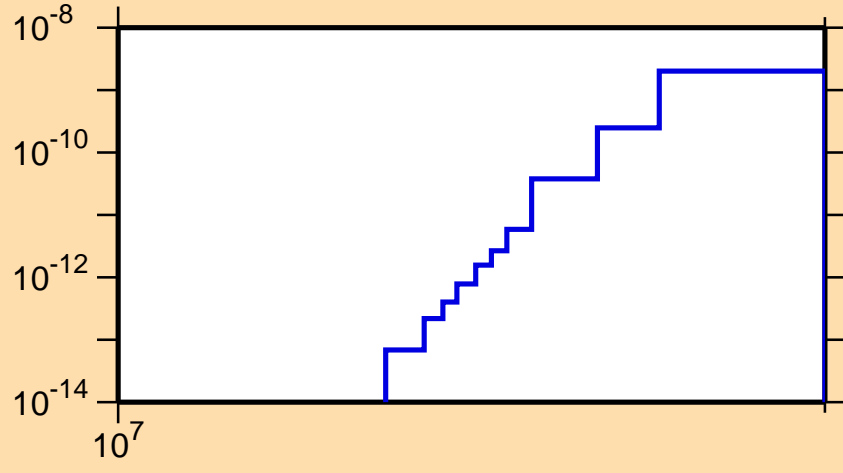
\sigma vs. E for ^{203}\text{Rn}(n,\text{pt})
