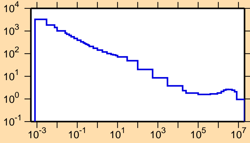
\sigma vs. E for ^{203}\text{Rn}(n,\gamma)
