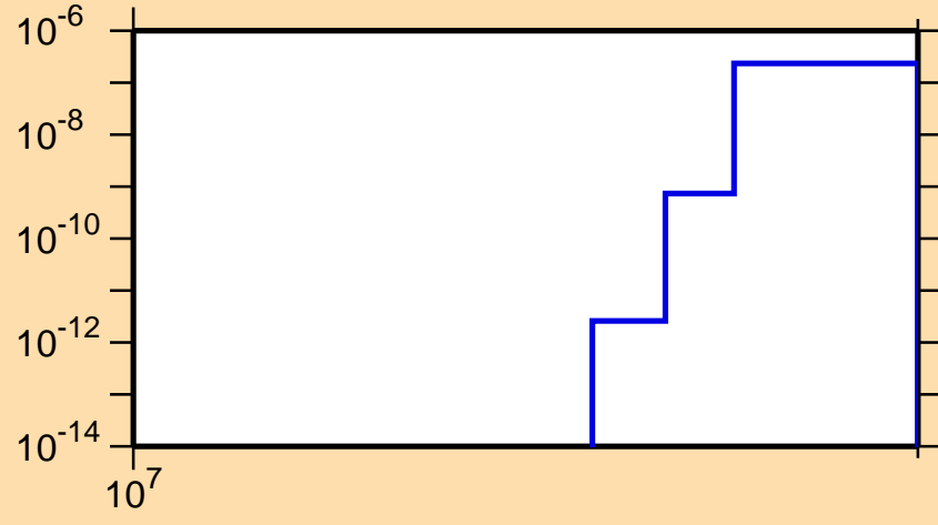
\sigma vs. E for ^{204}\text{Rn}(n,2np)
