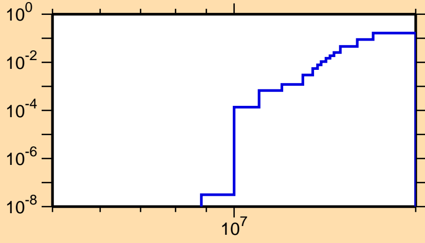
\sigma vs. E for ^{204}\text{Rn}(n,2n)
