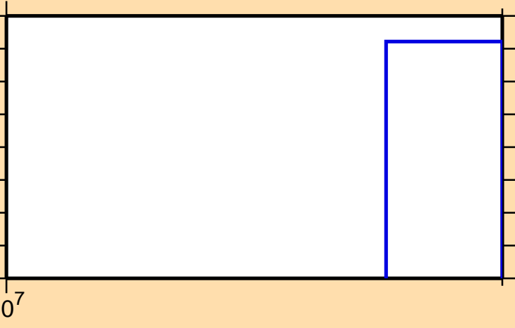
\sigma vs. E for ^{204}\text{Rn}(n,nt)
