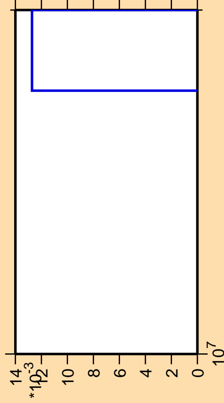
\Delta\sigma/\sigma vs. E for ^{204}\text{Rn}(n,3n\alpha)
