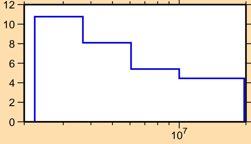
\Delta\sigma/\sigma vs. E for ^{204}\text{Rn}(n,n\text{onel.})
