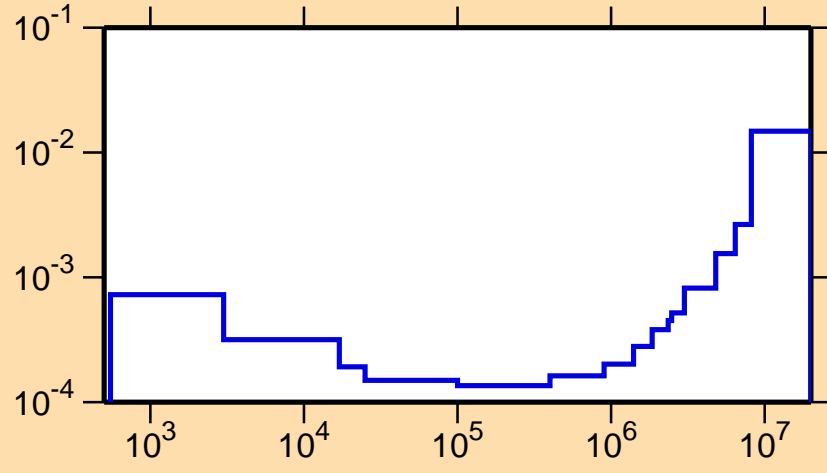
\sigma vs. E for ^{204}\text{Rn}(n,\alpha)
