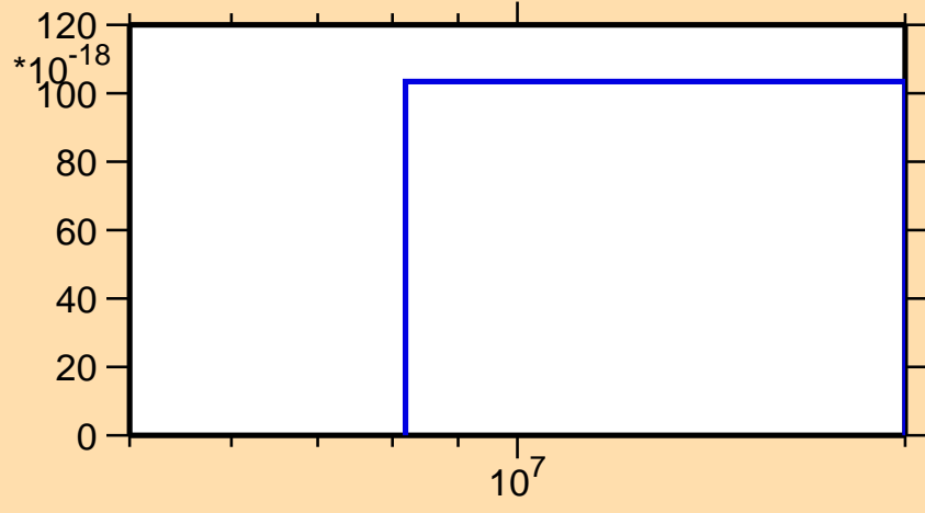
\sigma vs. E for ^{204}\text{Rn}(n,3n\alpha)
