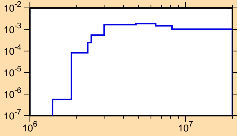
\sigma vs. E for ^{204}\text{Rn}(n,n_4)
