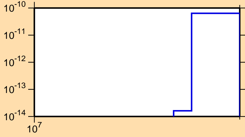
\sigma vs. E for ^{205}\text{Rn}(n,nt)
