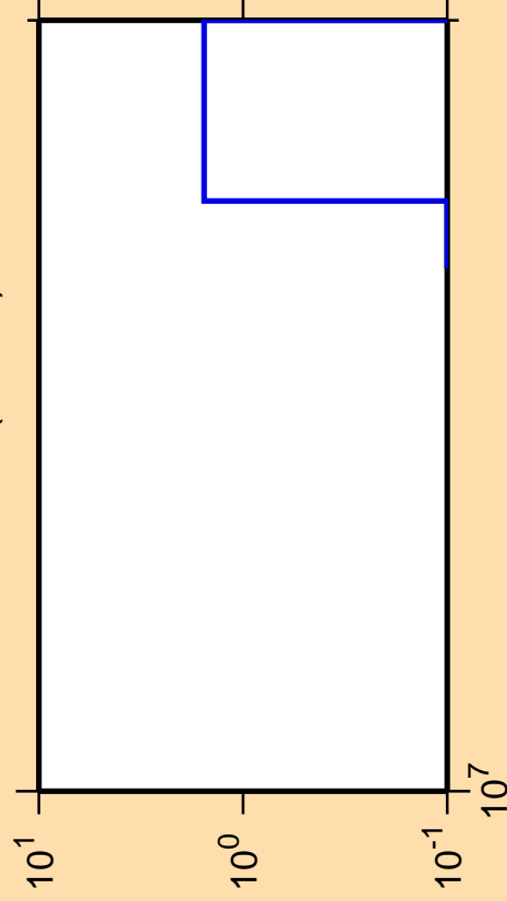
\Delta\sigma/\sigma vs. E for ^{205}\text{Rn}(n,3n\alpha)
