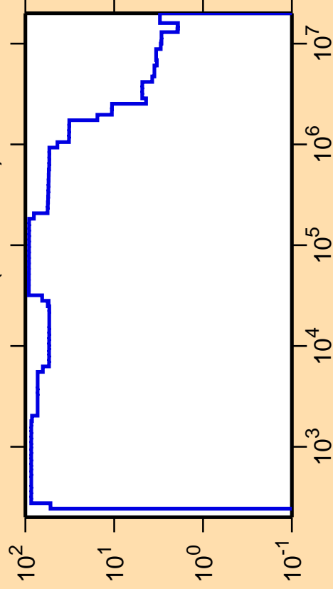
\Delta\sigma/\sigma vs. E for ^{205}\text{Rn}(n,\text{nonel.})
