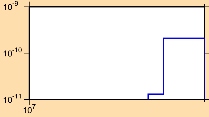
\sigma vs. E for ^{205}\text{Rn} (mt 34)
