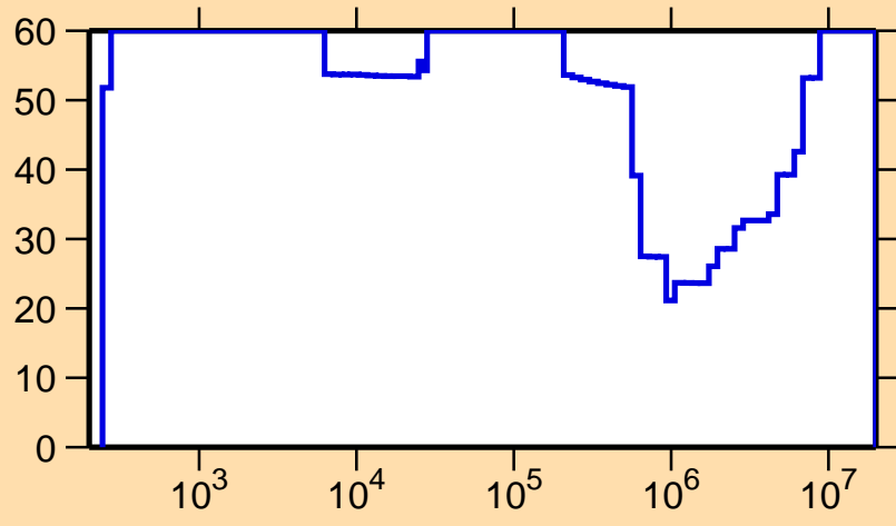
\Delta\sigma/\sigma vs. E for ^{205}\text{Rn}(n,\gamma)
