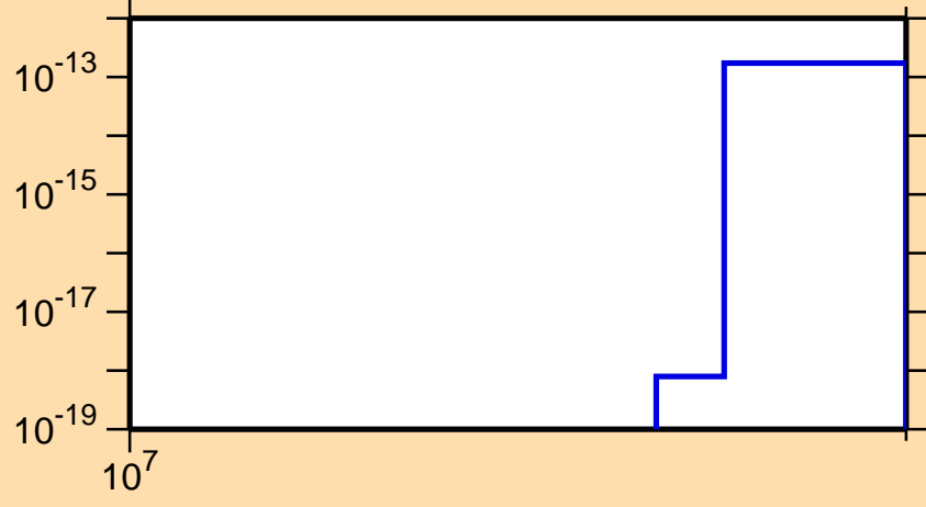
\sigma vs. E for ^{205}\text{Rn}(n,3n\alpha)
