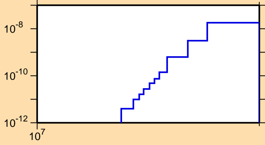
\sigma vs. E for ^{205}\text{Rn}(n,\text{pd})
