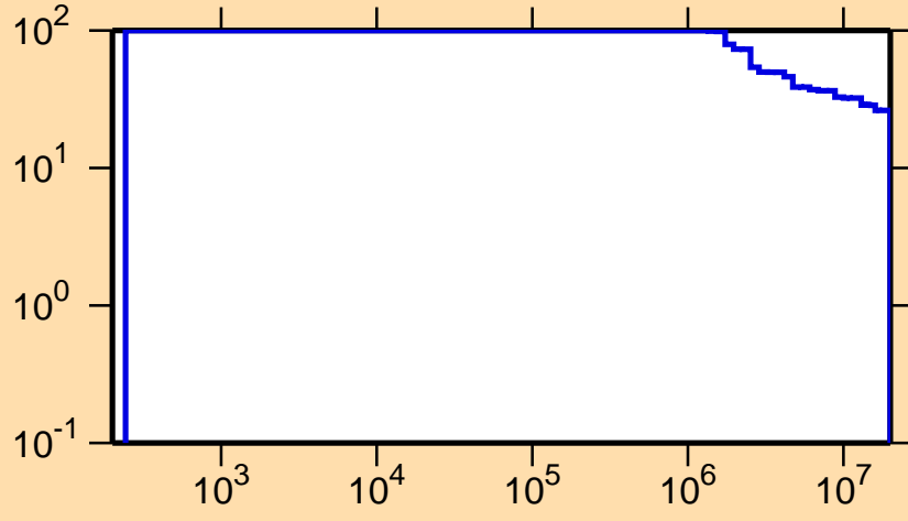
\Delta\sigma/\sigma vs. E for ^{205}\text{Rn}(n,p)
