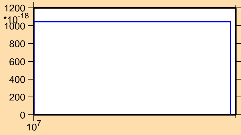
\sigma vs. E for ^{205}\text{Rn}(n,3n\alpha)
