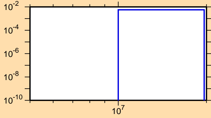
\sigma vs. E for ^{205}\text{Rn}(n,2n\alpha)
