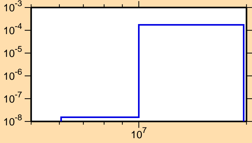
\sigma vs. E for ^{205}\text{Rn}(\text{mt } 45)
