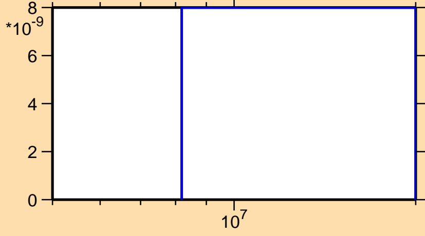
\sigma vs. E for ^{205}\text{Rn}(n,\text{nd})
