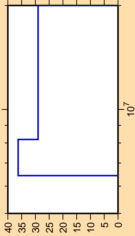
\Delta\sigma/\sigma vs. E for ^{205}\text{Rn}(n,p)
