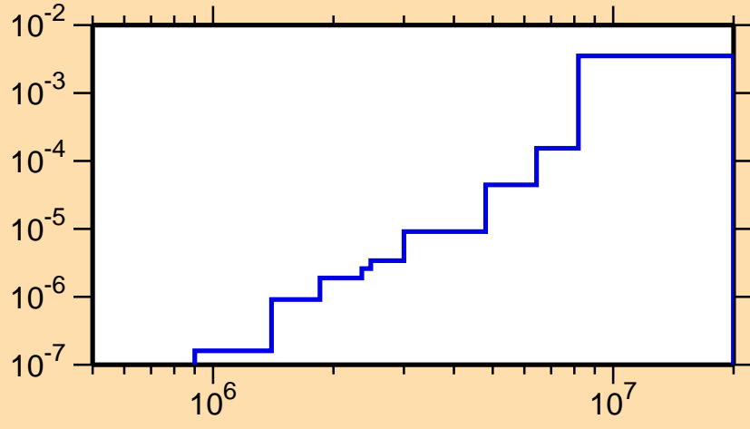
\sigma vs. E for ^{205}\text{Rn}(n,n\alpha)
