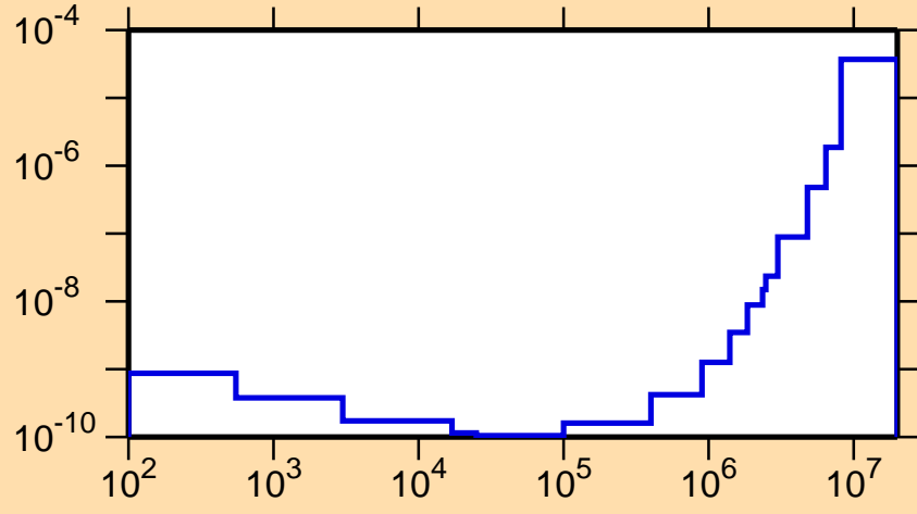
\sigma vs. E for ^{205}\text{Rn}(n,p\alpha)
