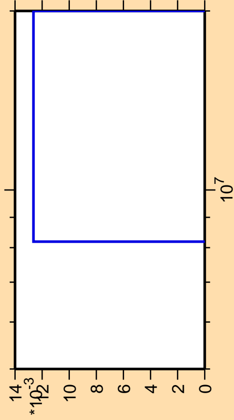
\Delta\sigma/\sigma vs. E for ^{205}\text{Rn}(n,3n\alpha)
