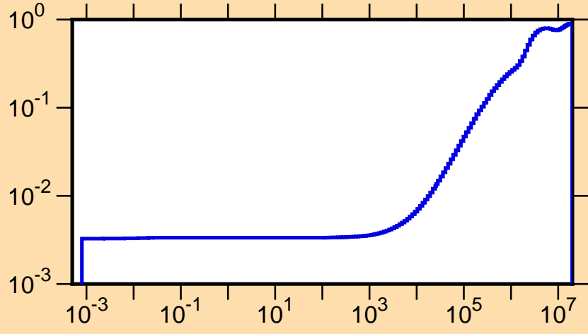
\mu vs. E for ^{206}\text{Rn}(\text{mt251})
