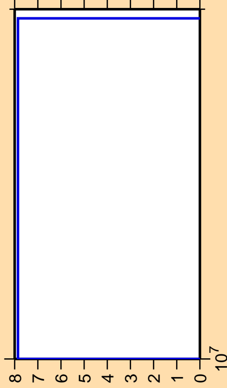
\Delta\sigma/\sigma vs. E for ^{206}\text{Rn}(n,nt)
