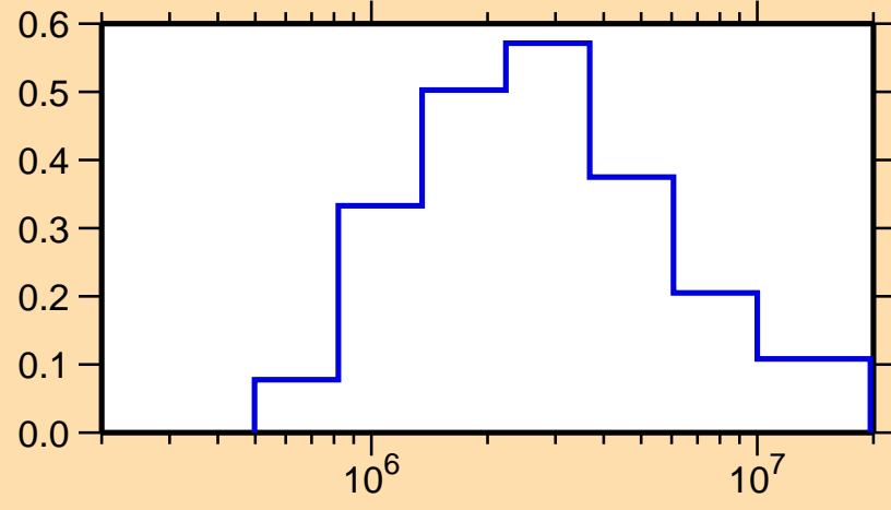
\sigma vs. E for ^{206}\text{Rn}(n,n_1)
