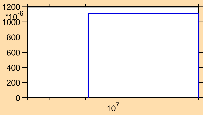
\sigma vs. E for ^{206}\text{Rn}(n,2n\alpha)
