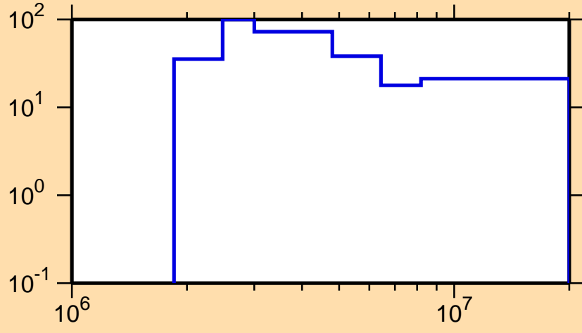
\Delta\sigma/\sigma vs. E for ^{206}\text{Rn}(n,n\text{cont.})
