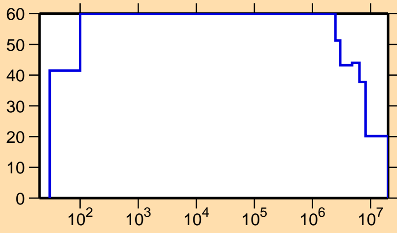
\Delta\sigma/\sigma vs. E for ^{206}\text{Rn}(n,p)
