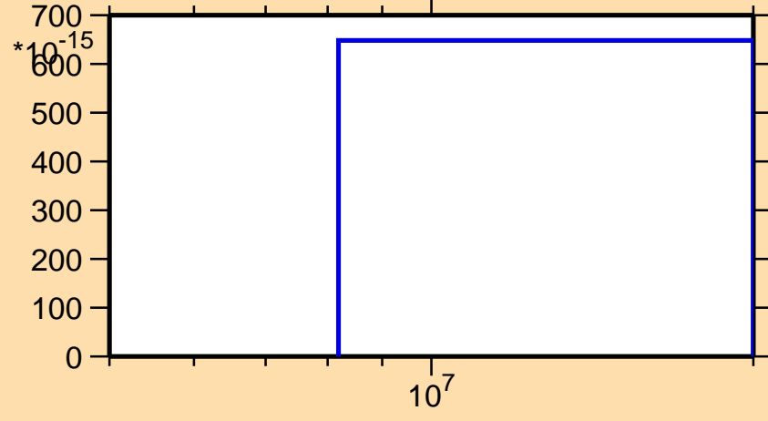
\sigma vs. E for ^{206}\text{Rn}(n,pt)
