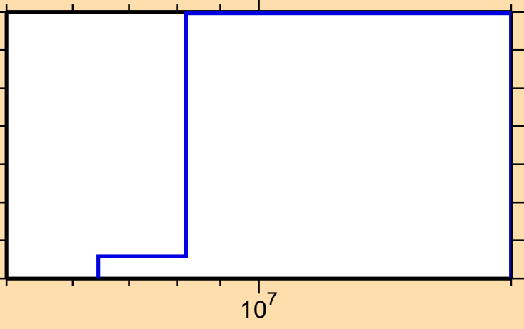
\sigma vs. E for ^{206}\text{Rn}(\text{mt117})
