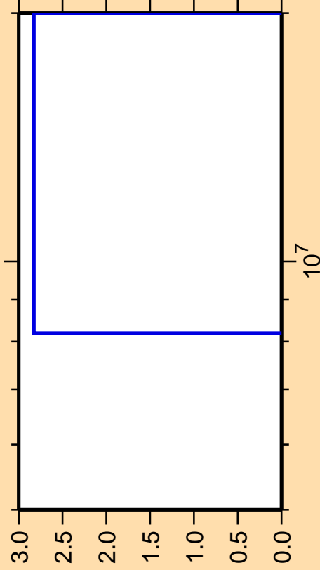
\Delta\sigma/\sigma vs. E for ^{206}\text{Rn}(n,pt)
