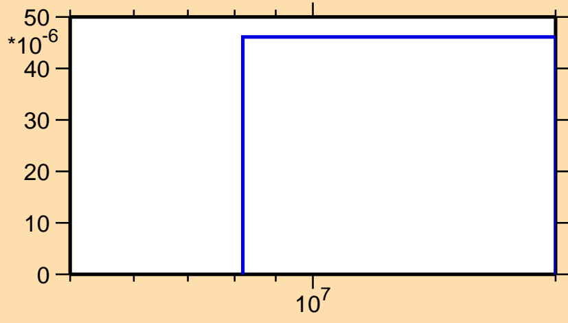
\sigma vs. E for ^{206}\text{Rn}(n,t)
