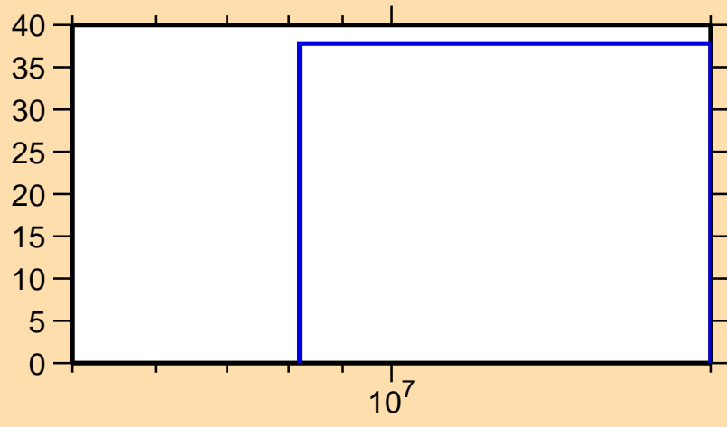
\Delta\sigma/\sigma vs. E for ^{206}\text{Rn}(n,2n)
