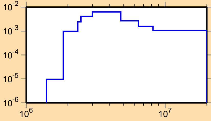
\sigma vs. E for ^{206}\text{Rn}(n,n_4)
