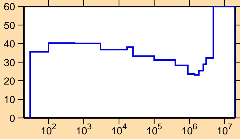
\Delta\sigma/\sigma vs. E for ^{206}\text{Rn}(n,\gamma)
