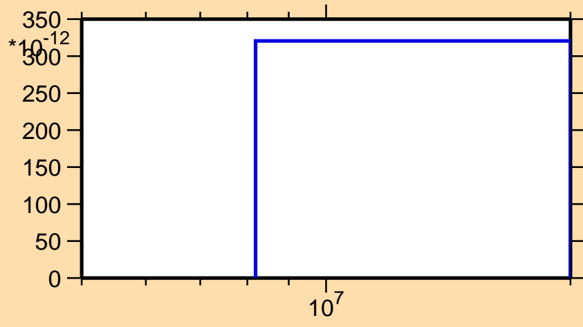
\sigma vs. E for ^{206}\text{Rn}(n,\text{pd})
