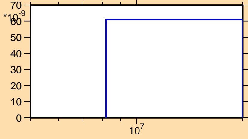
\sigma vs. E for ^{206}\text{Rn}(n,\text{He3})
