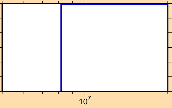
\sigma vs. E for ^{206}\text{Rn}(n,2np)
