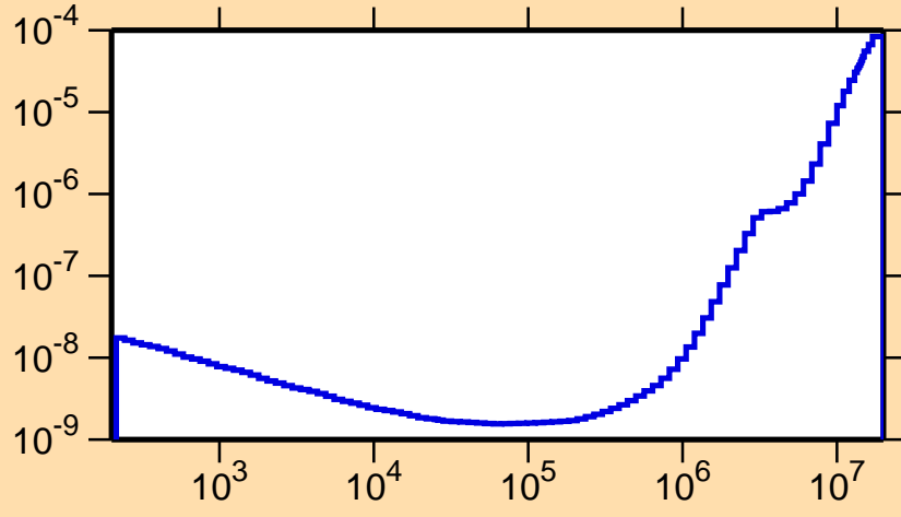
\sigma vs. E for ^{207}\text{Rn}(n,p\alpha)
