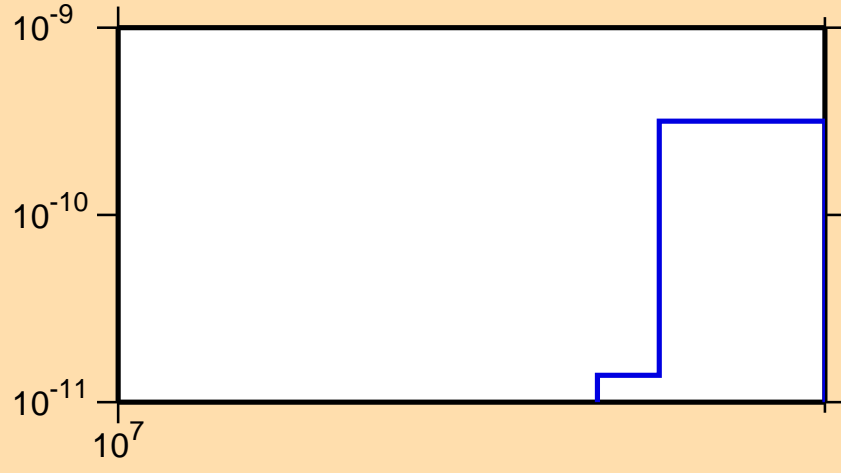
\sigma vs. E for ^{207}\text{Rn} (mt 34)
