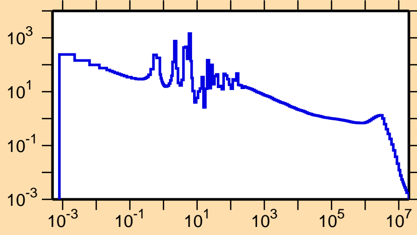
\sigma vs. E for ^{207}\text{Rn}(n,\gamma)
