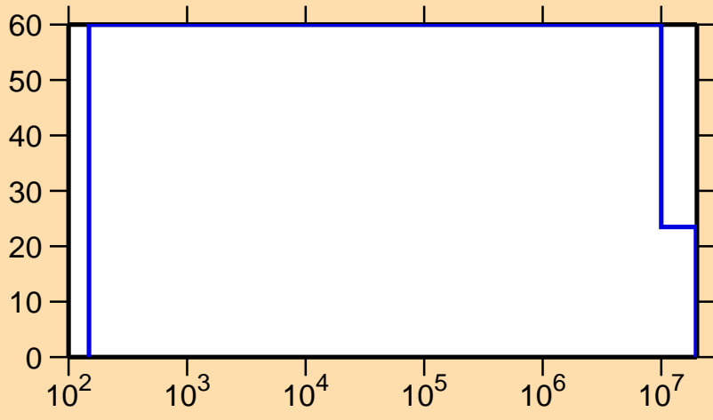
\Delta\sigma/\sigma vs. E for ^{207}\text{Rn}(n,p)
