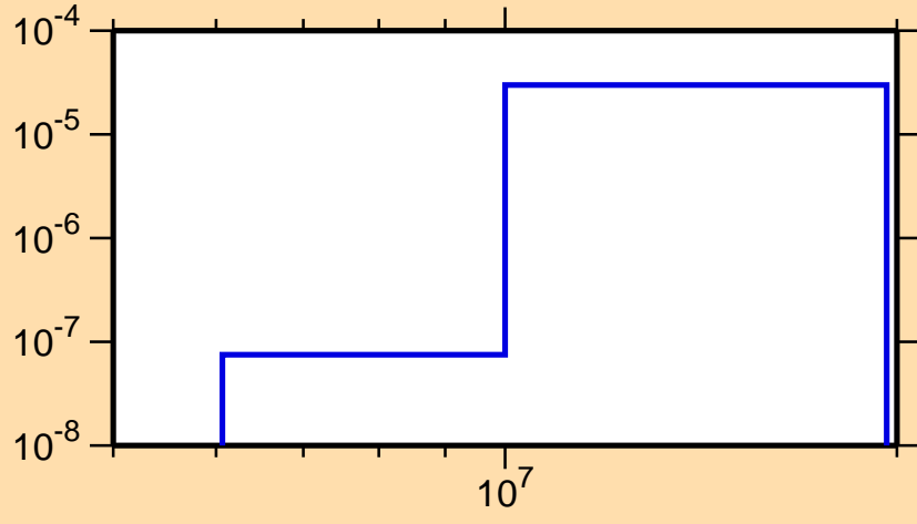
\sigma vs. E for ^{207}\text{Rn}(\text{mt } 45)
