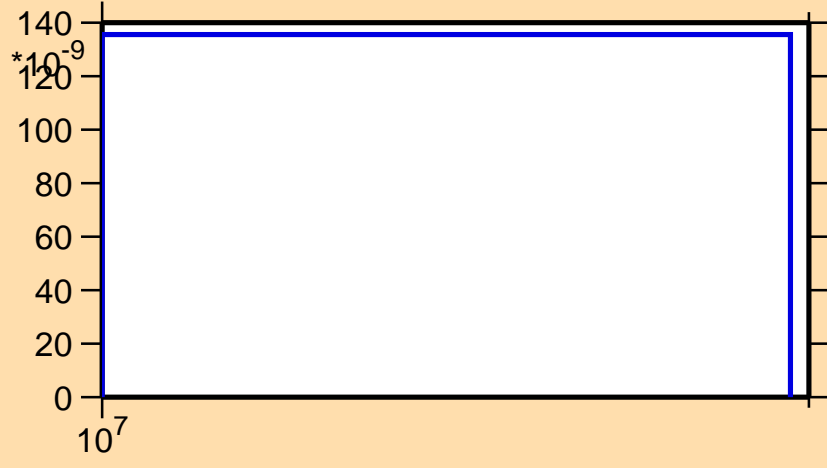
\sigma vs. E for ^{207}\text{Rn}(n,\text{nd})
