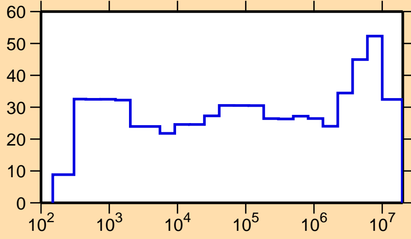
\Delta\sigma/\sigma vs. E for ^{207}\text{Rn}(n,\gamma)
