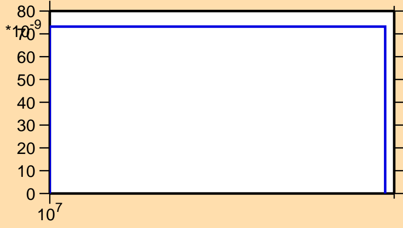
\sigma vs. E for ^{207}\text{Rn}(n,3n\alpha)
