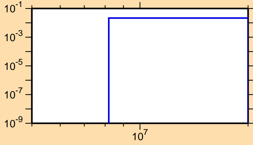
\sigma vs. E for ^{207}\text{Rn}(n,2n\alpha)
