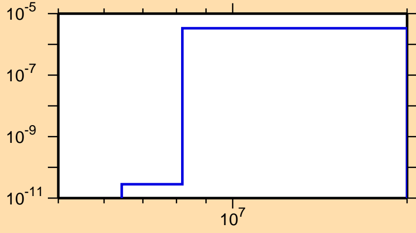
\sigma vs. E for ^{207}\text{Rn}(\text{mt117})
