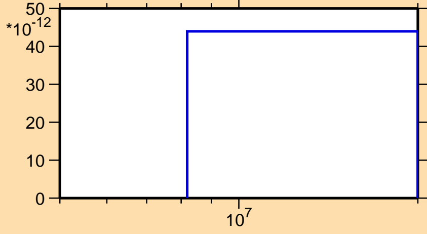
\sigma vs. E for ^{207}\text{Rn}(n,pt)
