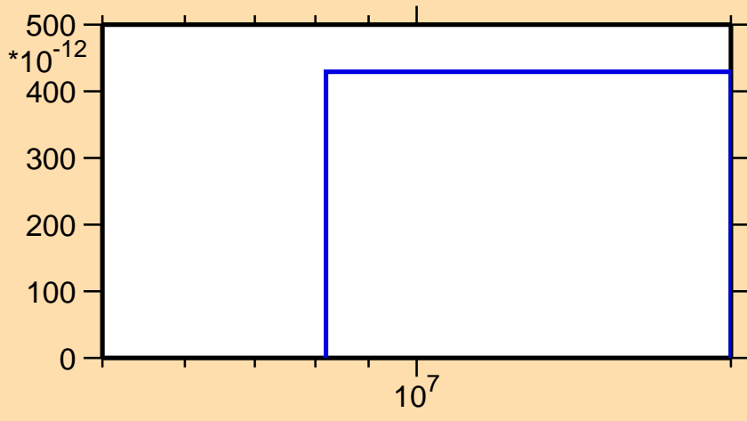
\sigma vs. E for ^{207}\text{Rn}(n,\text{pd})
