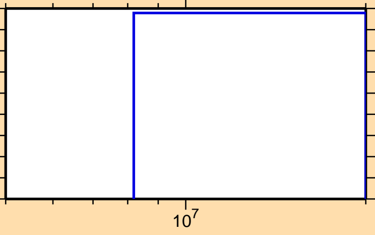
\sigma vs. E for ^{207}\text{Rn}(n,3n)
