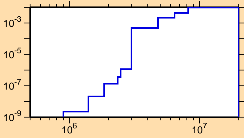
\sigma vs. E for ^{207}\text{Rn}(n,n\alpha)
