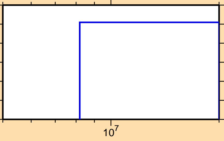
\sigma vs. E for ^{207}\text{Rn}(n,nt)
