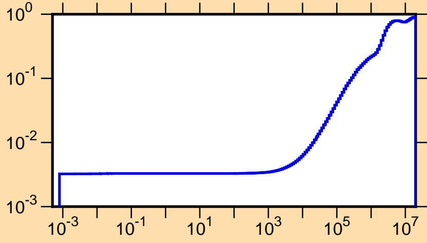
\mu vs. E for ^{208}\text{Rn}(\text{mt251})
