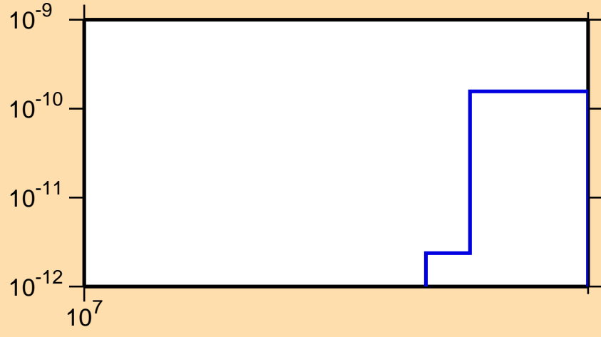
\sigma vs. E for ^{208}\text{Rn}(n,\text{pt})
