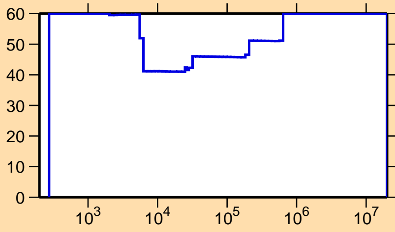
\Delta\sigma/\sigma vs. E for ^{208}\text{Rn}(n,\gamma)
