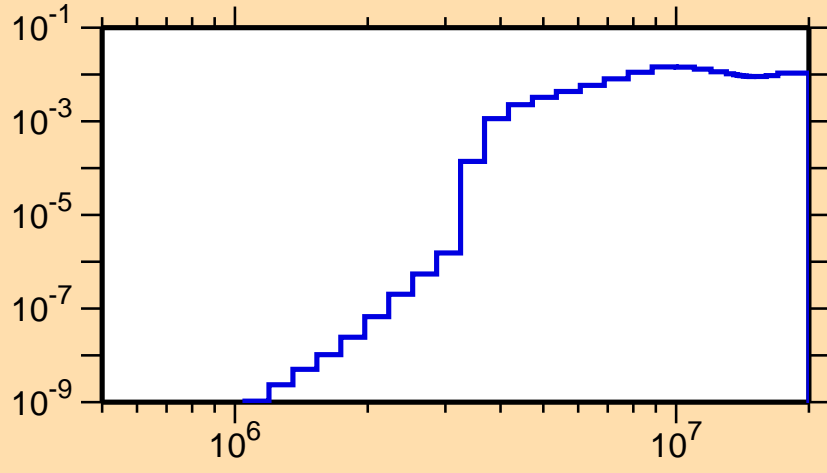
\sigma vs. E for ^{208}\text{Rn}(n,n\alpha)
