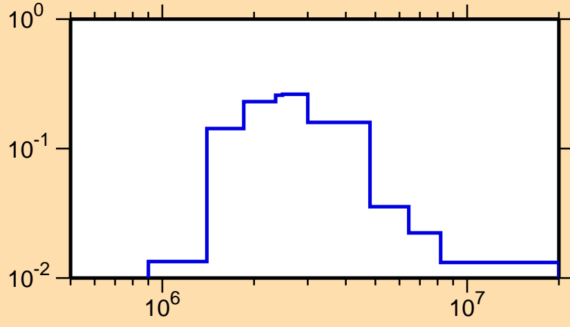
\sigma vs. E for ^{208}\text{Rn}(n,n_2)
