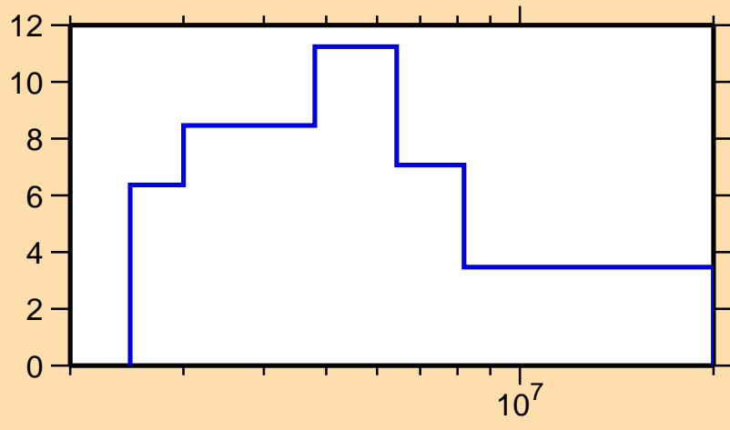
\Delta\sigma/\sigma vs. E for ^{208}\text{Rn}(n,\text{tot.})
