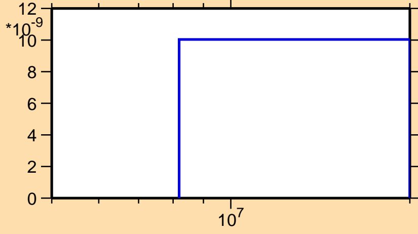
\sigma vs. E for ^{208}\text{Rn}(n,nd)
