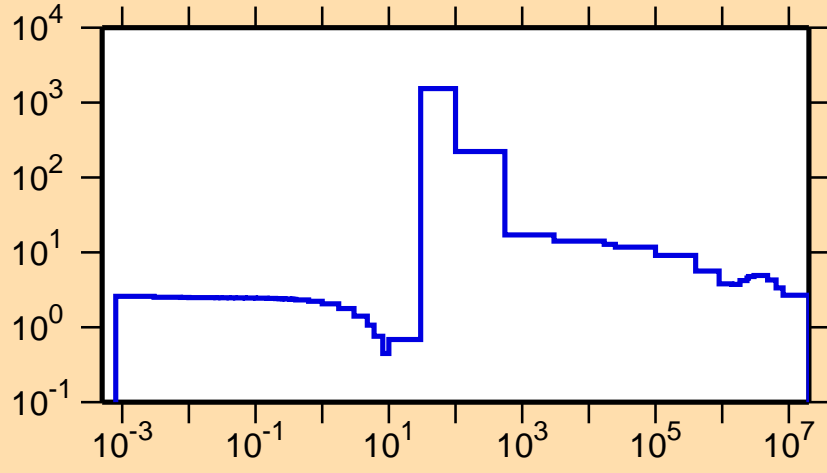
\sigma vs. E for ^{208}\text{Rn}(n,\text{el.})
