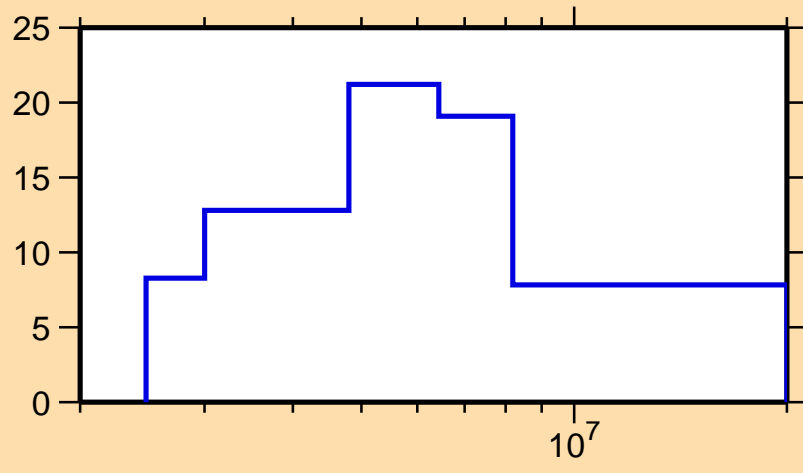
\Delta\sigma/\sigma vs. E for ^{208}\text{Rn}(n,\text{el.})
