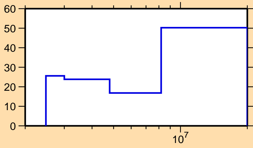
\Delta\sigma/\sigma vs. E for ^{208}\text{Rn}(n,n\text{cont.})
