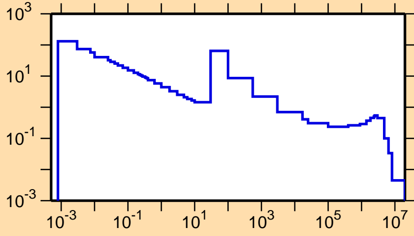
\sigma vs. E for ^{208}\text{Rn}(n,\gamma)
