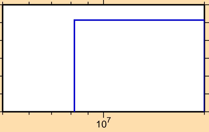
\sigma vs. E for ^{208}\text{Rn}(n,t)
