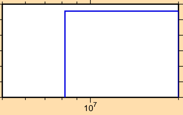
\sigma vs. E for ^{209}\text{Rn}(n,\text{He3})
