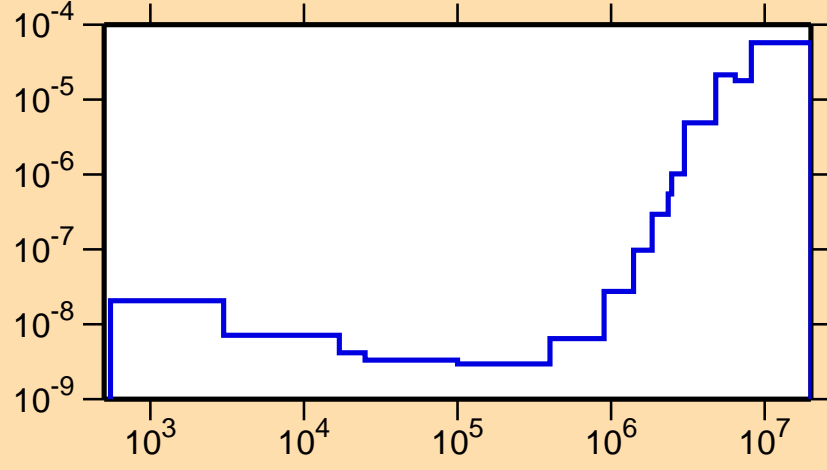
\sigma vs. E for ^{209}\text{Rn}(n,p\alpha)
