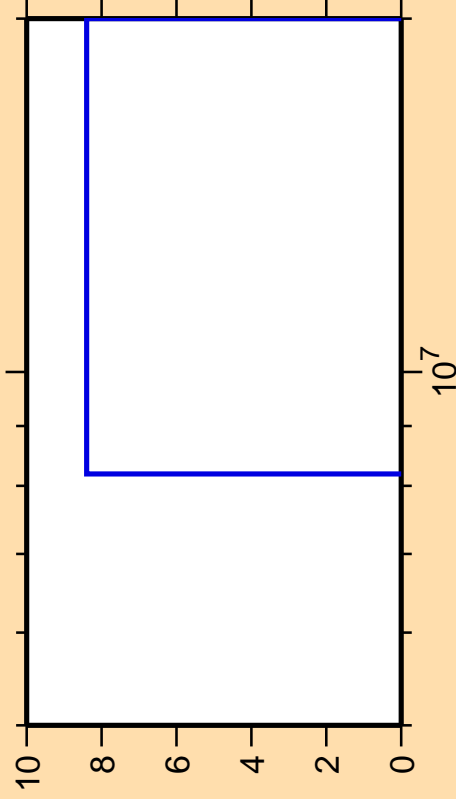
\Delta\sigma/\sigma vs. E for ^{209}\text{Rn}(\text{mt } 34)
