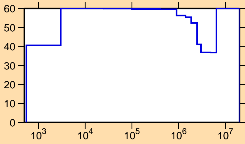
\Delta\sigma/\sigma vs. E for ^{209}\text{Rn}(n,\gamma)
