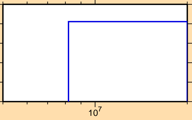
\sigma vs. E for ^{209}\text{Rn}(n,2np)
