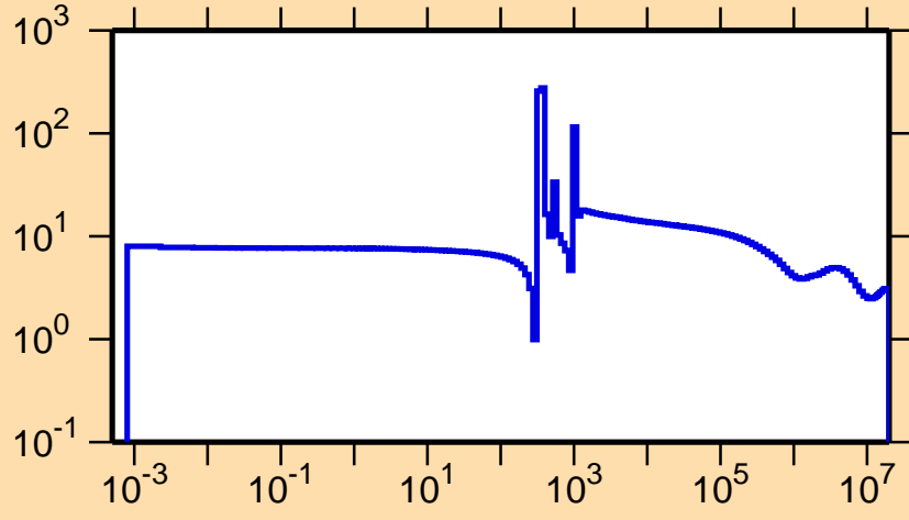
\sigma vs. E for ^{210}\text{Rn}(n,\text{el.})
