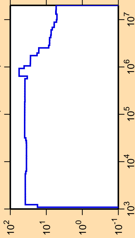
\Delta\sigma/\sigma vs. E for ^{210}\text{Rn}(n,\text{nonel.})
