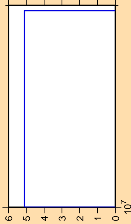
\Delta\sigma/\sigma vs. E for ^{210}\text{Rn}(n,\text{pt})
