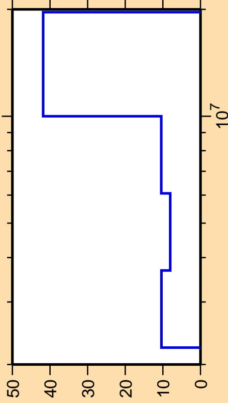
\Delta\sigma/\sigma vs. E for ^{211}\text{Rn}(n,n_{\text{cont}}) .
