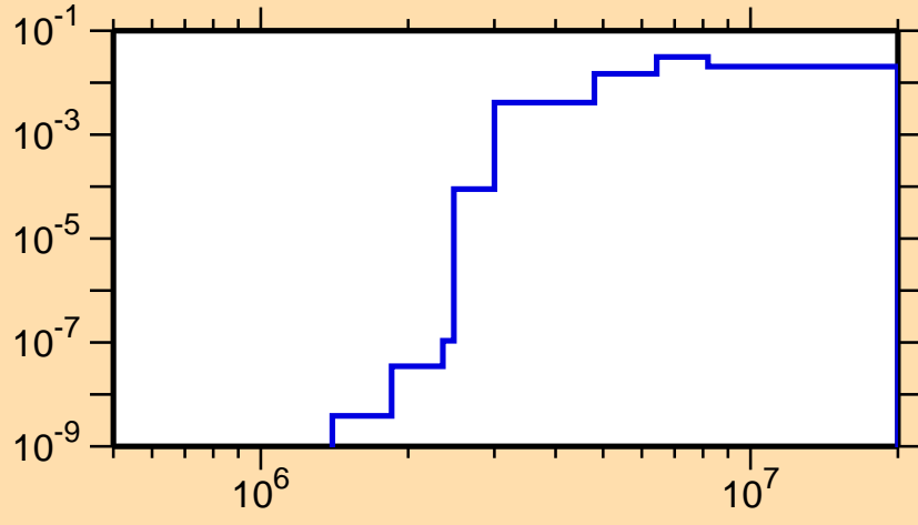
\sigma vs. E for ^{211}\text{Rn}(n,n\alpha)
