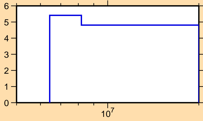
\Delta\sigma/\sigma vs. E for ^{211}\text{Rn}(n,\text{nonel.})
