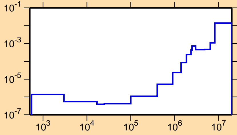
\sigma vs. E for ^{211}\text{Rn}(n,p)
