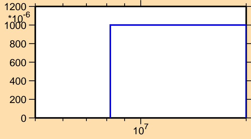
\sigma vs. E for ^{211}\text{Rn}(n,3n)
