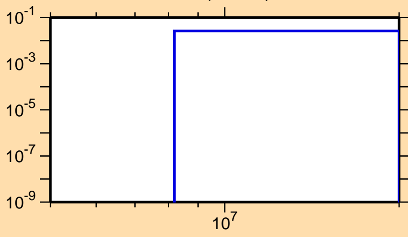
\sigma vs. E for ^{211}\text{Rn}(n,2n\alpha)
