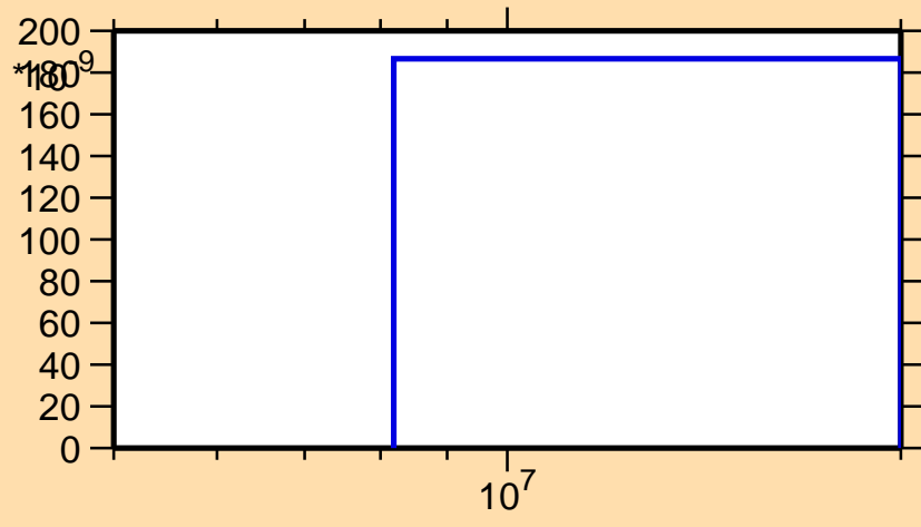
\sigma vs. E for ^{211}\text{Rn}(n,nd)
