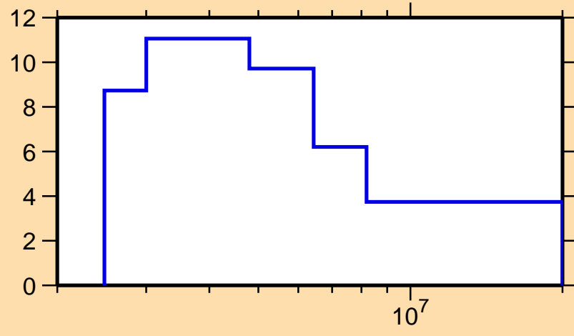
\Delta\sigma/\sigma vs. E for ^{211}\text{Rn}(n,\text{tot.})
