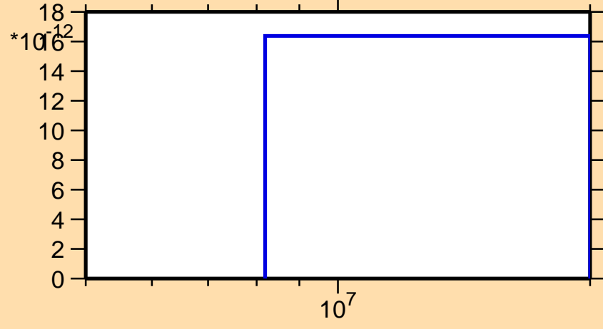
\sigma vs. E for ^{211}\text{Rn}(n,\text{pt})
