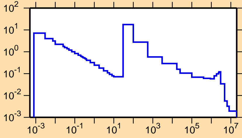
\sigma vs. E for ^{211}\text{Rn}(n,\gamma)
