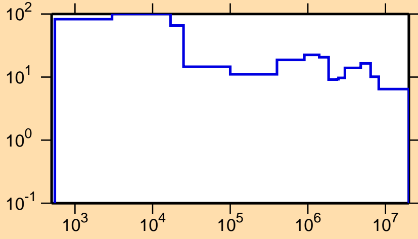
\Delta\sigma/\sigma vs. E for ^{211}\text{Rn}(n,\text{el.})
