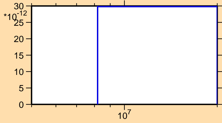
\sigma vs. E for ^{211}\text{Rn}(n,\text{pd})
