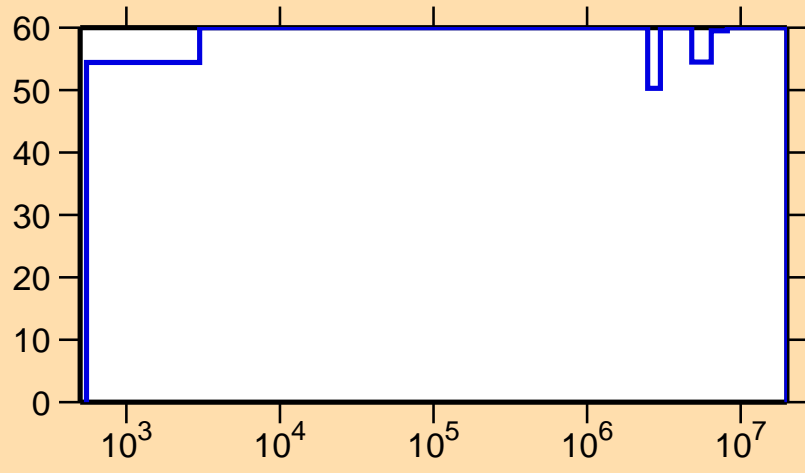
\Delta\sigma/\sigma vs. E for ^{211}\text{Rn}(n,\gamma)
