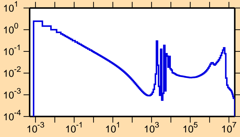
\sigma vs. E for ^{212}\text{Rn}(n,\gamma)
