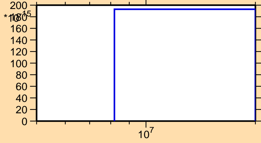
\sigma vs. E for ^{212}\text{Rn}(n,pt)
