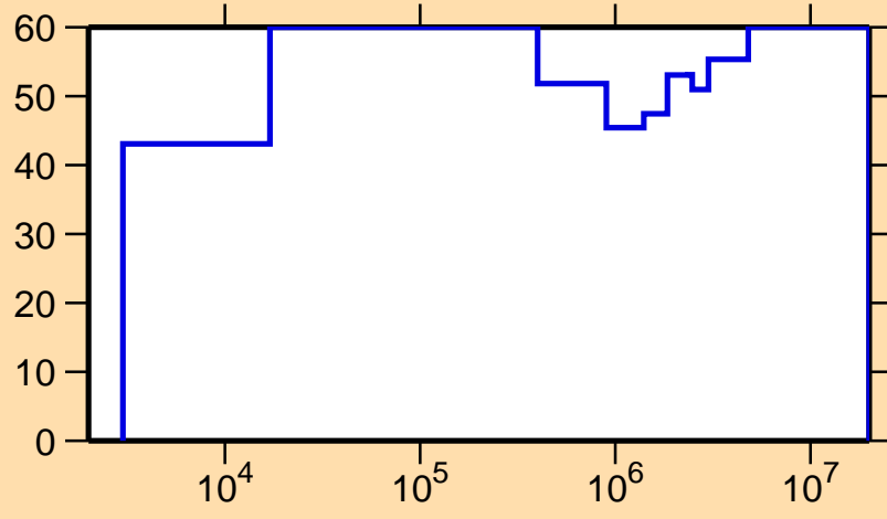
\Delta\sigma/\sigma vs. E for ^{212}\text{Rn}(n,\gamma)
