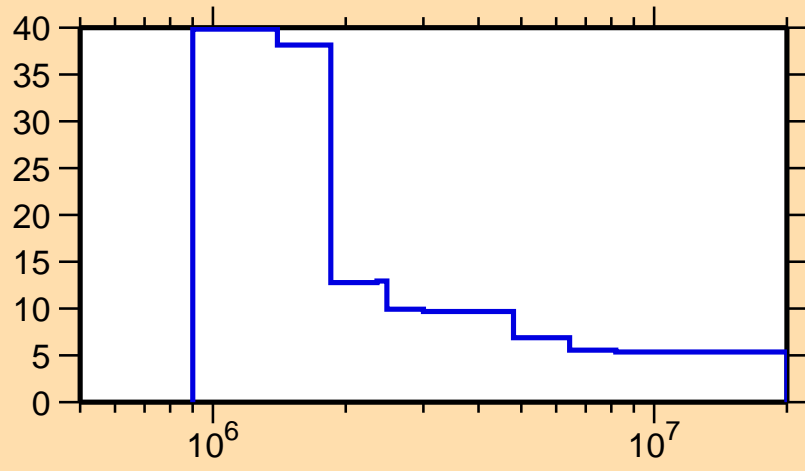
\Delta\sigma/\sigma vs. E for ^{212}\text{Rn}(n,\text{nonel.})
