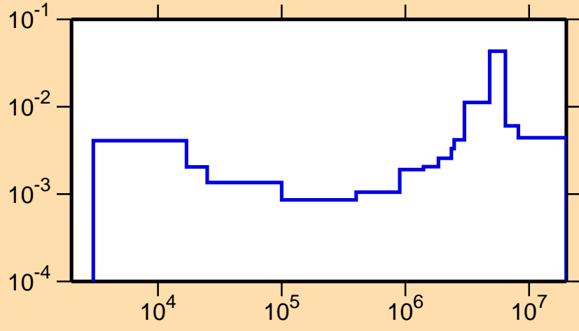
\sigma vs. E for ^{212}\text{Rn}(n,\alpha)
