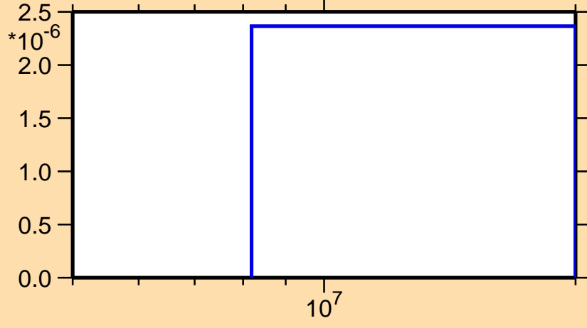
\sigma vs. E for ^{212}\text{Rn}(n,3n\alpha)
