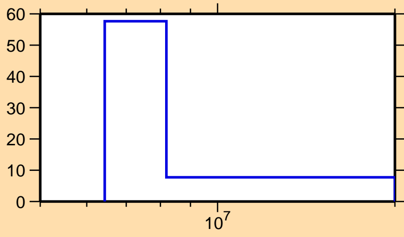
\Delta\sigma/\sigma vs. E for ^{212}\text{Rn}(n,2n)
