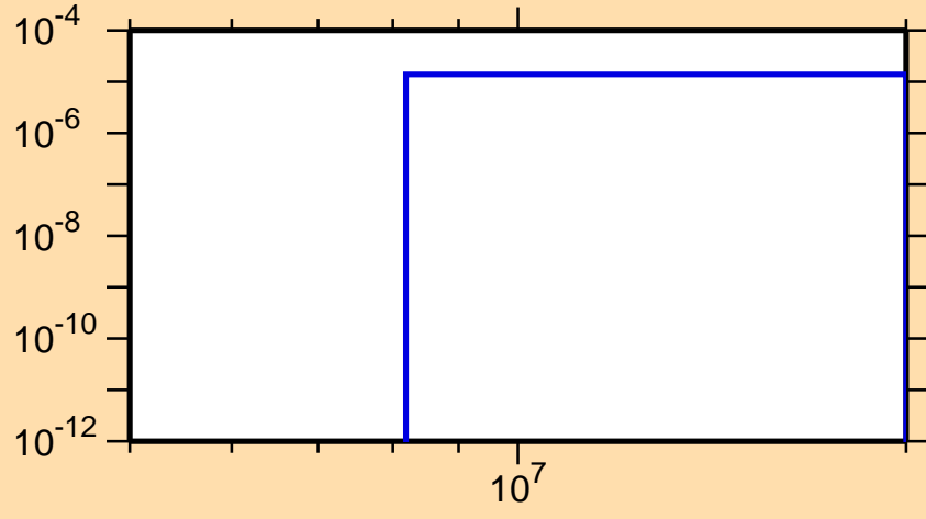
\sigma vs. E for ^{212}\text{Rn}(\text{mt117})
