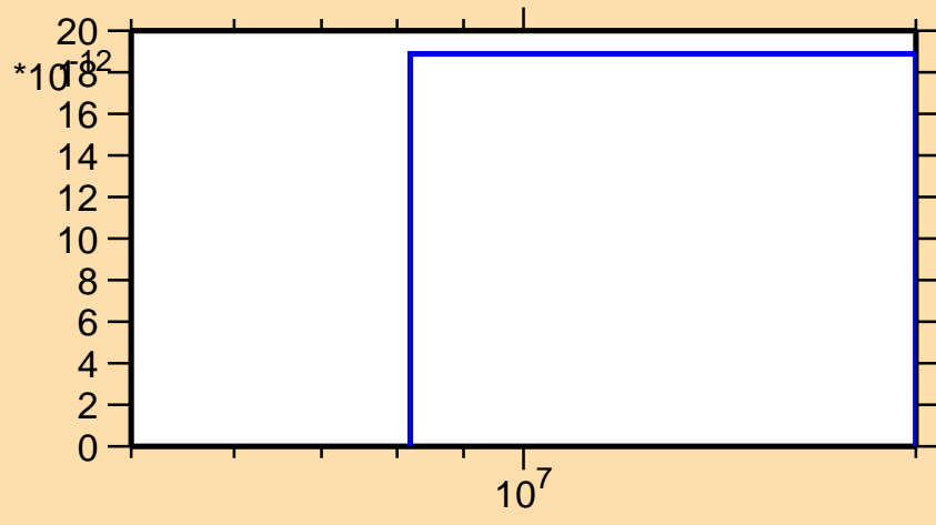
\sigma vs. E for ^{212}\text{Rn}(n,\text{pd})
