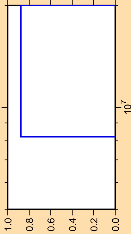
\Delta\sigma/\sigma vs. E for ^{212}\text{Rn}(n,pt)
