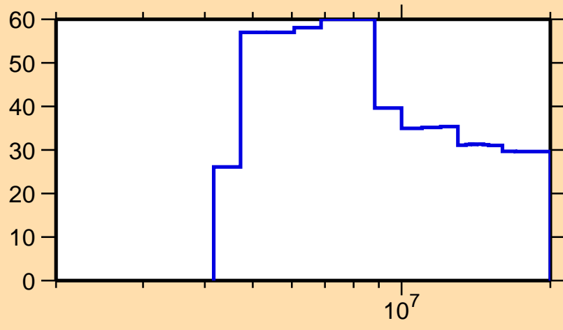
\Delta\sigma/\sigma vs. E for ^{219}\text{Rn}(n,\text{inel.})
