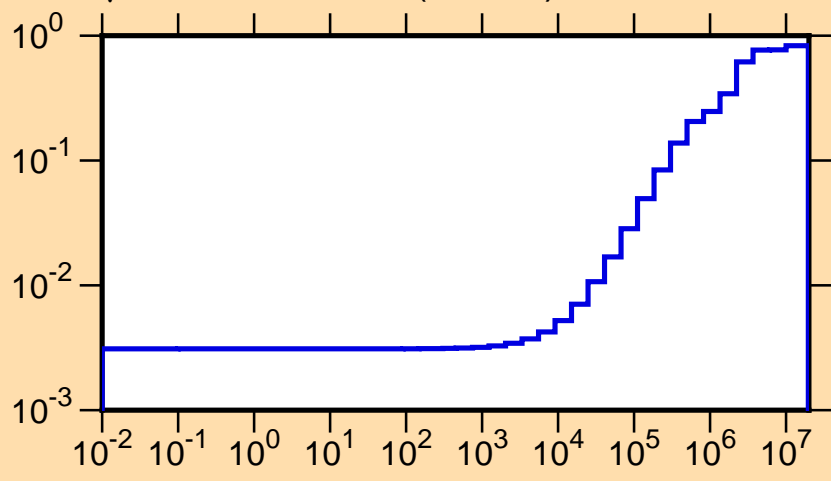
\mu vs. E for ^{219}\text{Rn}(\text{mt251})
