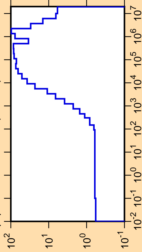
\Delta\mu/\mu vs. E for ^{219}\text{Rn}(\text{mt251})
