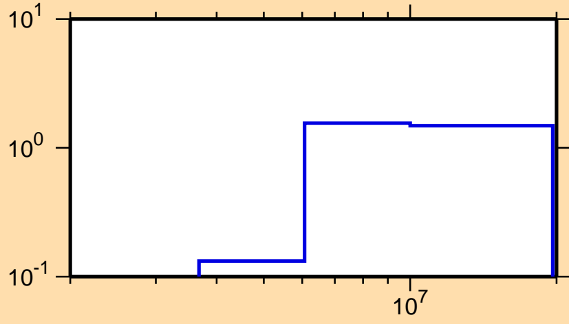
\sigma vs. E for ^{219}\text{Rn}(n,2n)
