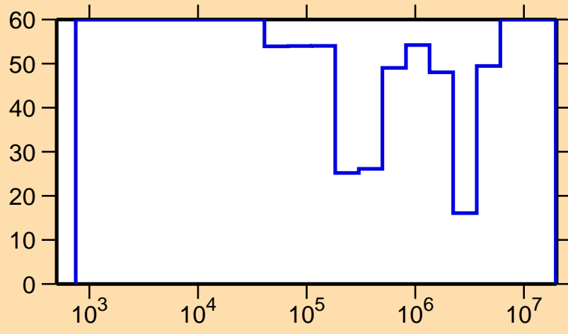
\Delta\sigma/\sigma vs. E for ^{219}\text{Rn}(n,\gamma)
