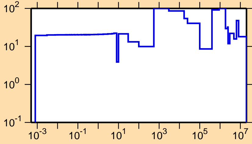
\Delta\sigma/\sigma vs. E for ^{219}\text{Rn}(n,el.)
