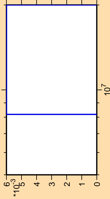
\Delta\sigma/\sigma vs. E for ^{219}\text{Rn} (mt 42)
