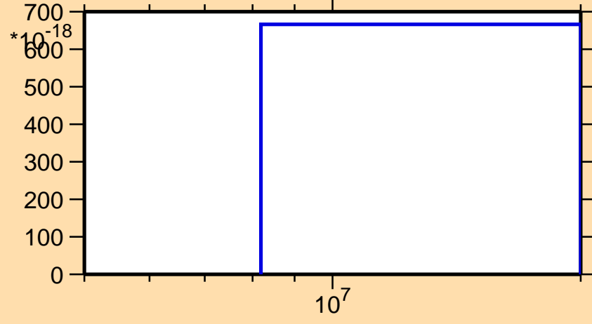
\sigma vs. E for ^{219}\text{Rn} (mt 42)
