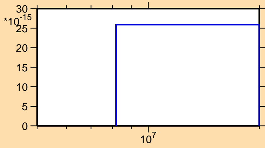
\sigma vs. E for ^{219}\text{Rn} (mt 11)
