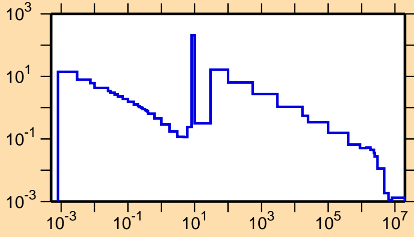
\sigma vs. E for ^{219}\text{Rn}(n,\gamma)
