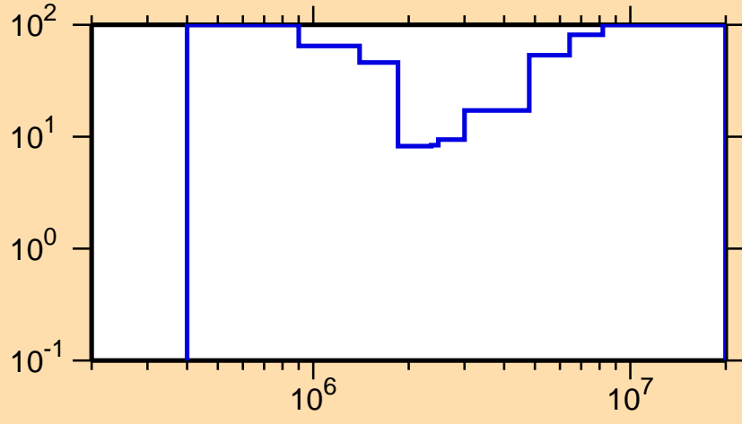
\Delta\sigma/\sigma vs. E for ^{219}\text{Rn}(n,n\text{cont.})
