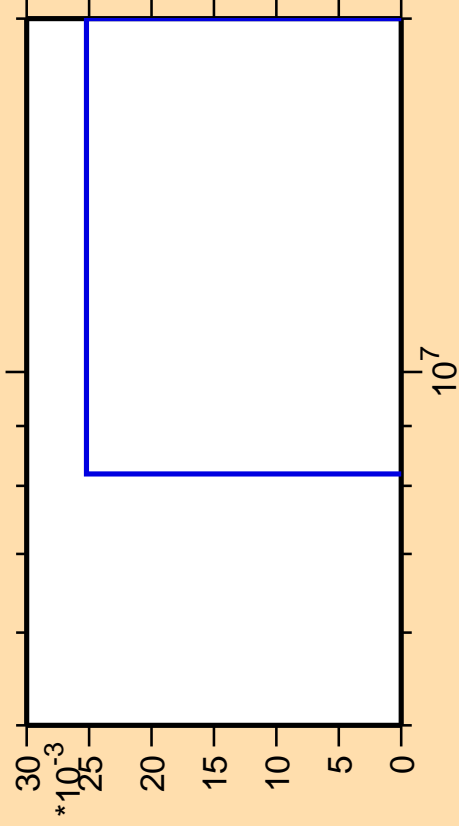
\Delta\sigma/\sigma vs. E for ^{219}\text{Rn} (mt 11)
