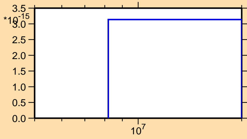
\sigma vs. E for ^{219}\text{Rn} (mt 34)
