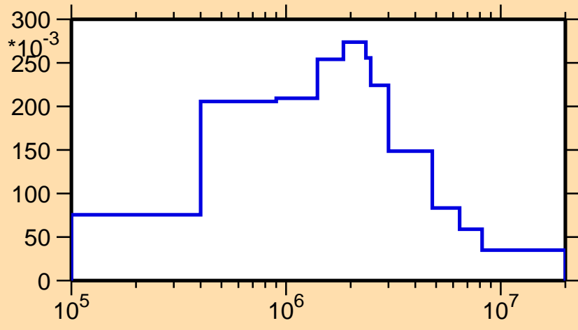
\sigma vs. E for ^{219}\text{Rn}(n,n_4)
