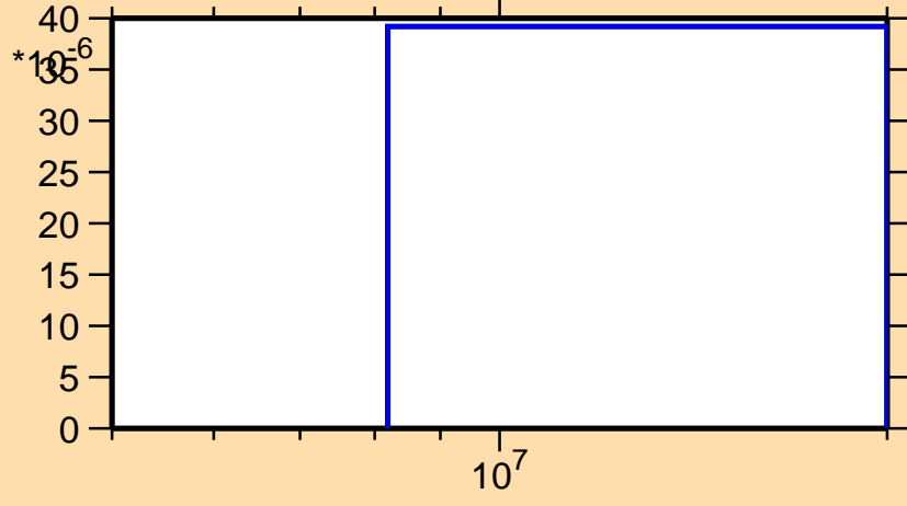
\sigma vs. E for ^{219}\text{Rn}(n,np)
