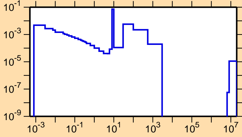
\sigma vs. E for ^{219}\text{Rn}(n,f)
