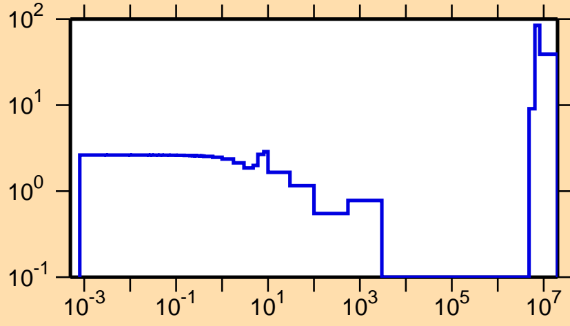
\Delta\sigma/\sigma vs. E for ^{219}\text{Rn}(n,f)
