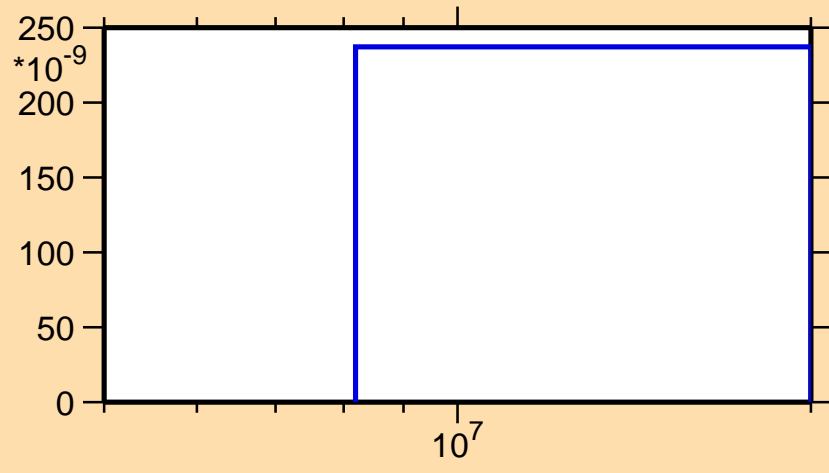
\sigma vs. E for ^{219}\text{Rn}(n,nd)
