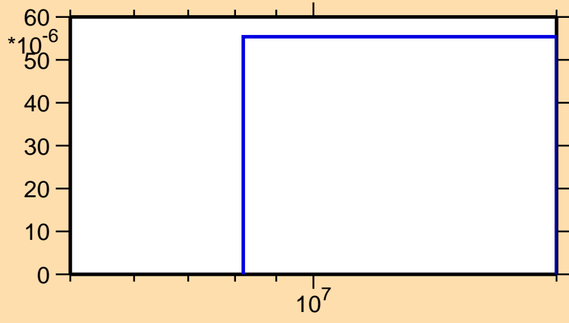
\sigma vs. E for ^{219}\text{Rn}(\text{mt117})
