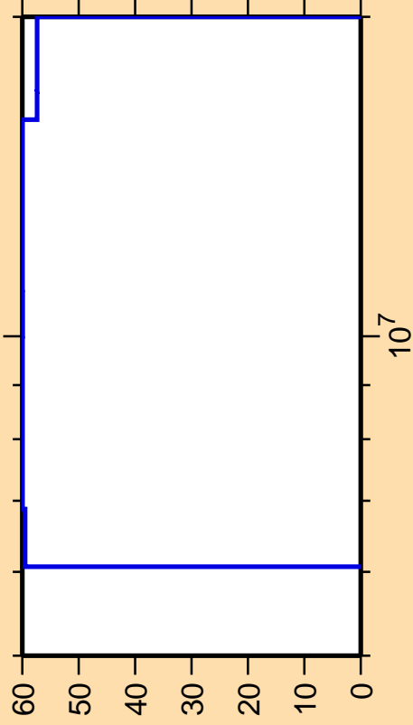
\Delta\sigma/\sigma vs. E for ^{220}\text{Rn}(n,n_1)
