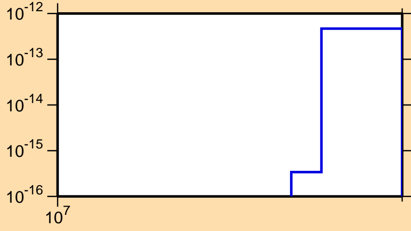
\sigma vs. E for ^{220}\text{Rn} (mt 11)
