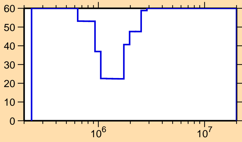
\Delta\sigma/\sigma vs. E for ^{220}\text{Rn}(n,\text{inel.})
