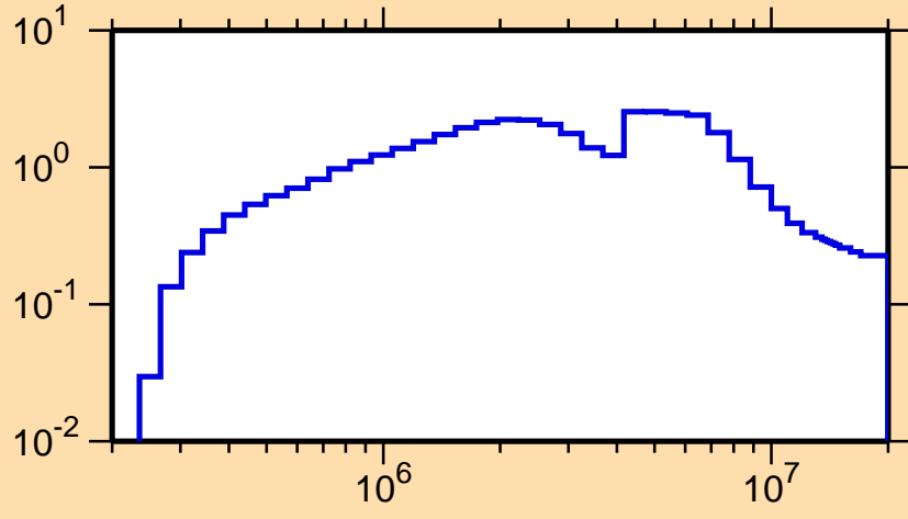
\sigma vs. E for ^{220}\text{Rn}(n,\text{inel.})
