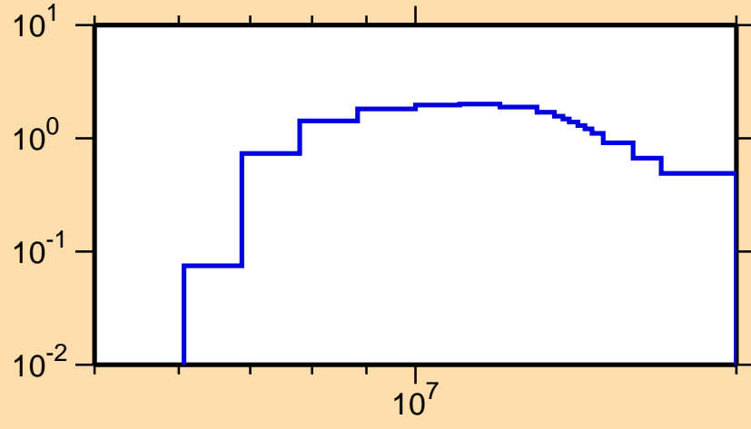
\sigma vs. E for ^{220}\text{Rn}(n,2n)
