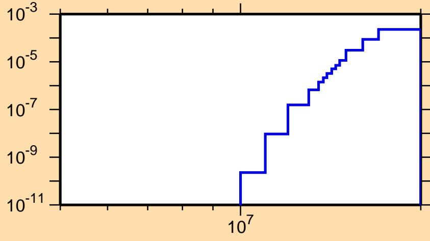
\sigma vs. E for ^{220}\text{Rn}(\text{mt117})
