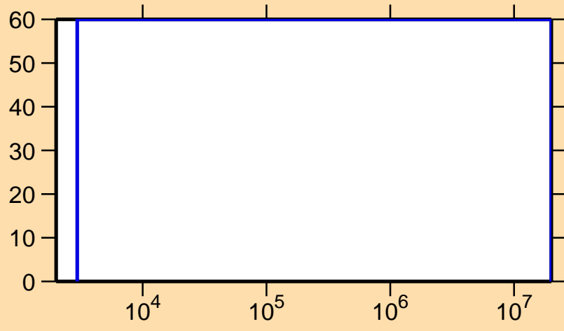
\Delta\sigma/\sigma vs. E for ^{220}\text{Rn}(n,\gamma)
