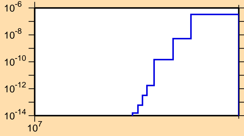
\sigma vs. E for ^{220}\text{Rn}(n,\text{nd})
