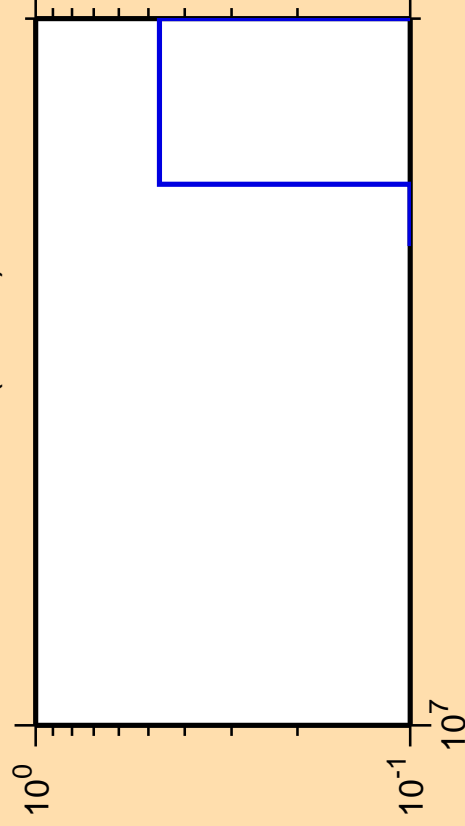
\Delta\sigma/\sigma vs. E for ^{220}\text{Rn} (mt 11)
