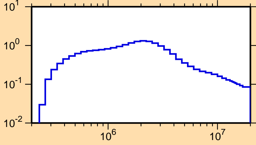
\sigma vs. E for ^{220}\text{Rn}(n,n_1)
