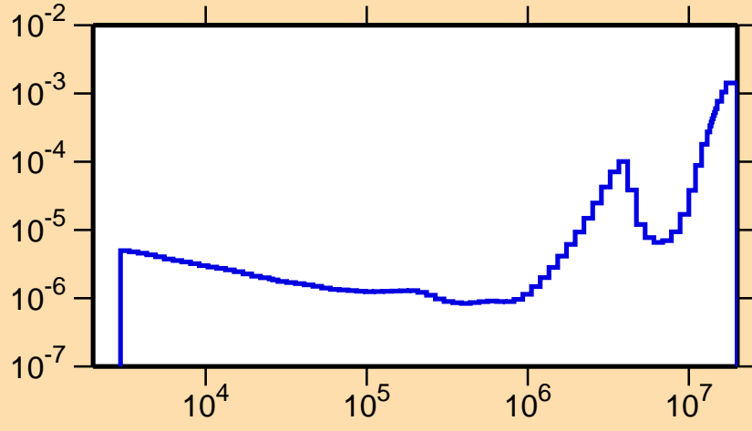
\sigma vs. E for ^{220}\text{Rn}(n,\alpha)
