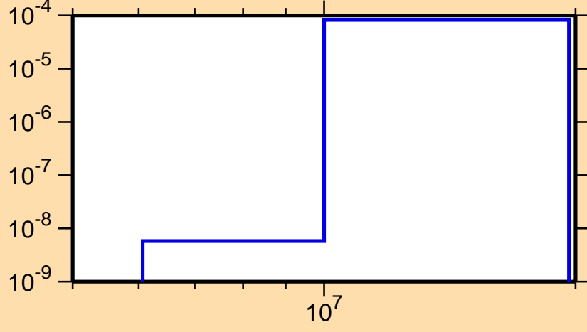
\sigma vs. E for ^{220}\text{Rn}(n,p\alpha)
