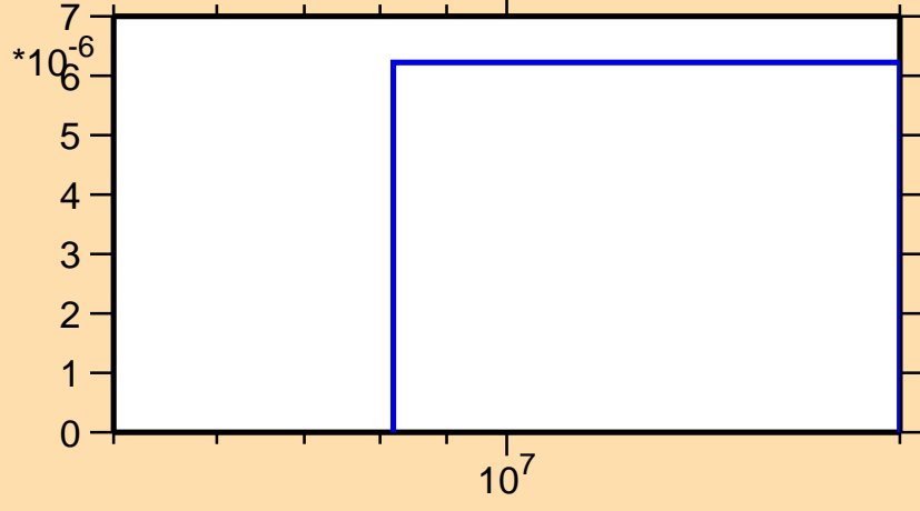
\sigma vs. E for ^{220}\text{Rn}(\text{mt } 45)
