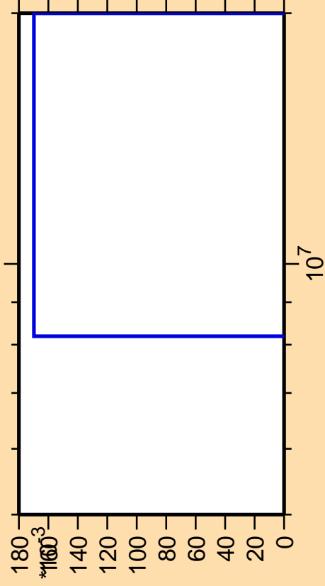
\Delta\sigma/\sigma vs. E for ^{220}\text{Rn}(n,\text{He}3)
