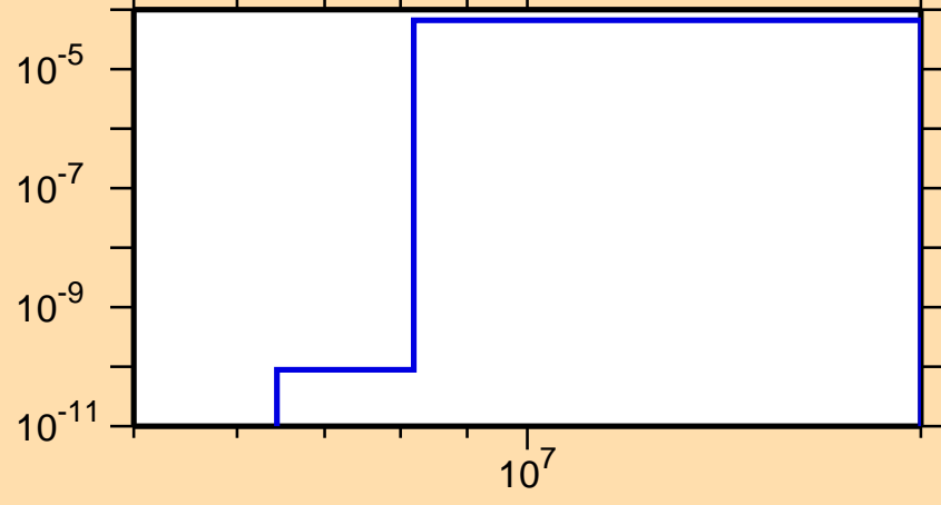
\sigma vs. E for ^{220}\text{Rn}(n,p\alpha)
