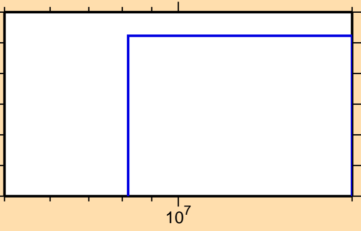
\sigma vs. E for ^{220}\text{Rn}(n,2np)
