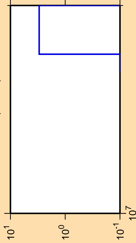
\Delta\sigma/\sigma vs. E for ^{221}\text{Rn} (mt 11)
