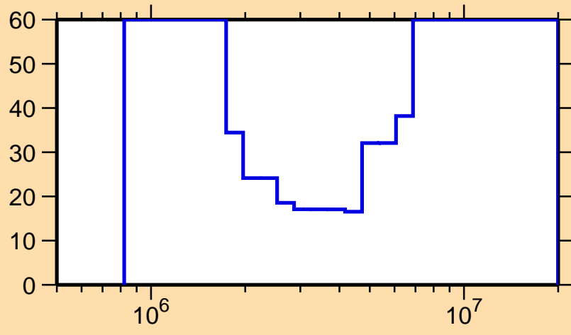
\Delta\sigma/\sigma vs. E for ^{221}\text{Rn}(n,n\text{cont.})
