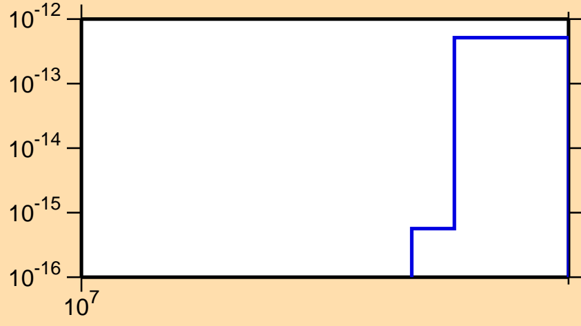
\sigma vs. E for ^{221}\text{Rn} (mt 11)
