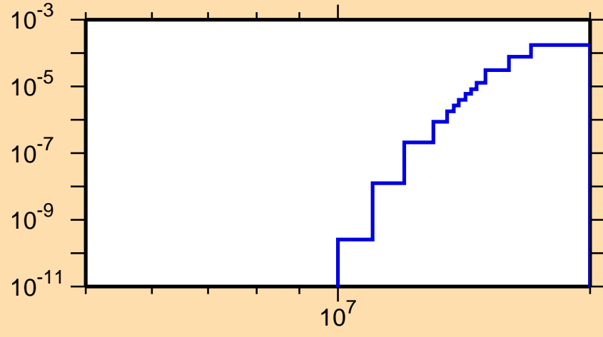
\sigma vs. E for ^{221}\text{Rn}(\text{mt117})
