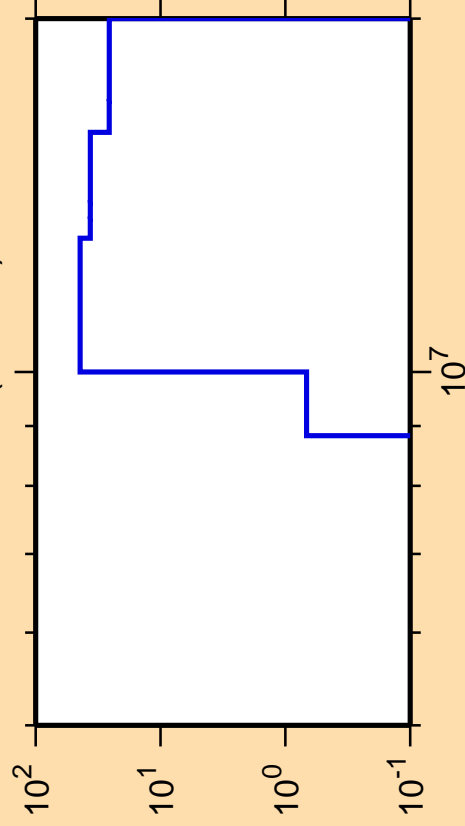
\Delta\sigma/\sigma vs. E for ^{221}\text{Rn}(\text{mt117})
