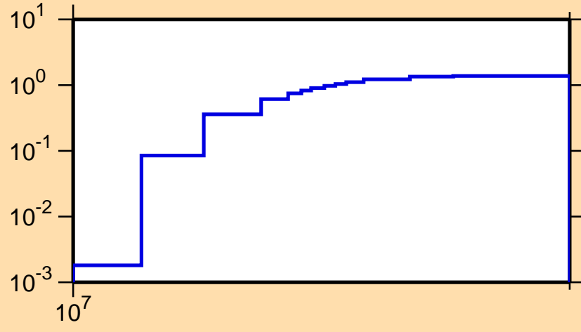
\sigma vs. E for ^{221}\text{Rn}(n,3n)
