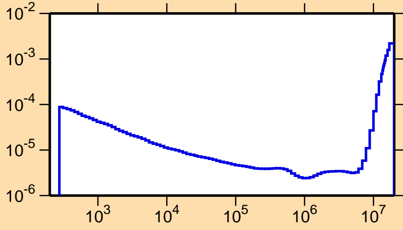
\sigma vs. E for ^{221}\text{Rn}(n,\alpha)
